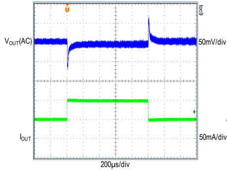
LOAD TRANSIENT RESPONSE, LOAD CURRENT STEPPED FROM 50mA to 100mA, FIGURE 3 CIRCUIT
