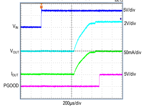
STARTUP RESPONSE WITH 100mA LOAD FIGURE 3 CIRCUIT
