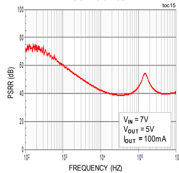
POWER SUPPLY REJECTION RATIO, FIGURE 3 CIRCUIT
