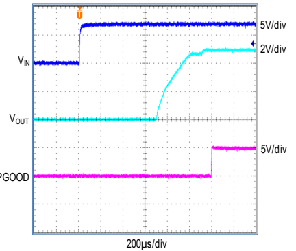
STARTUP RESPONSE WITH NO LOAD FIGURE 3 CIRCUIT
