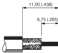
Part Number: 192945-4530
