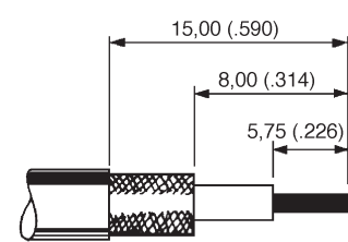
Part Number: 192945-4530
