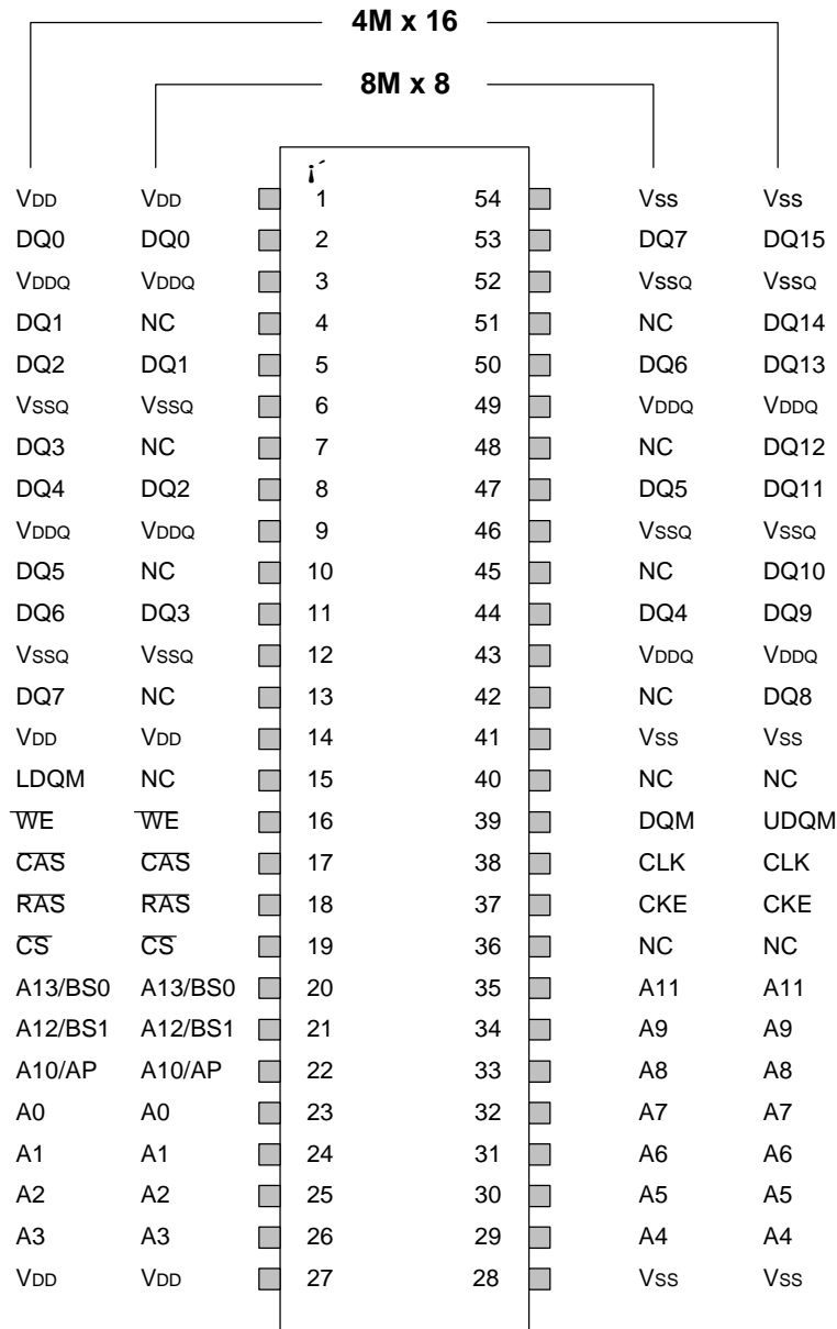
54-pin Plastic TSOP-II 400 mil
