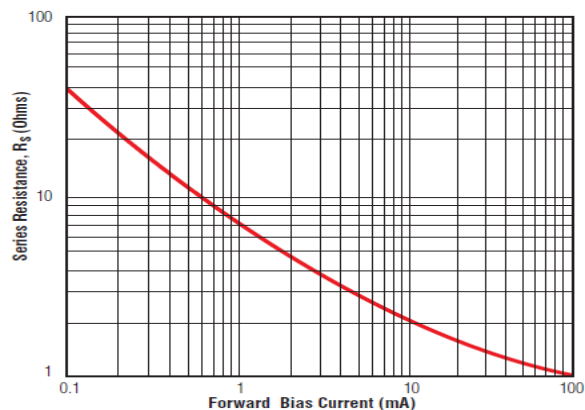
SMPN7310, @ 1 GHz
