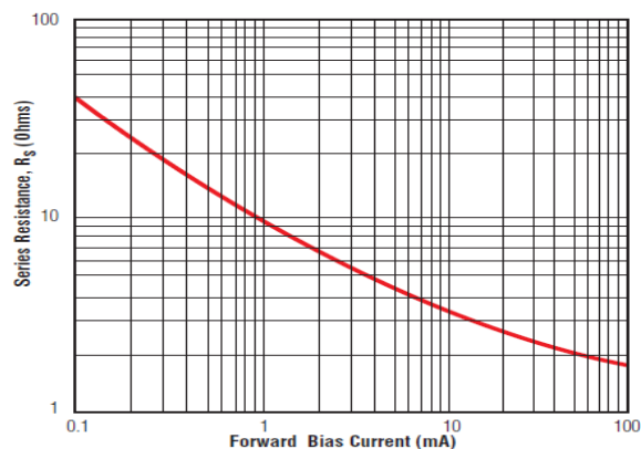
SMPN7320, @ 1 GHz
