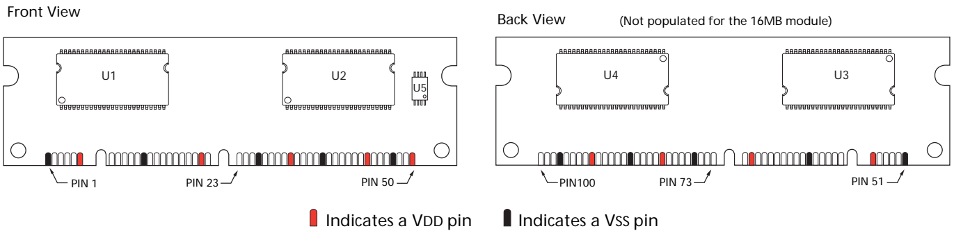
Figure 2: Module Layout
