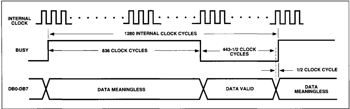
Figure 11. Conversion Timing, Continuous Mode
