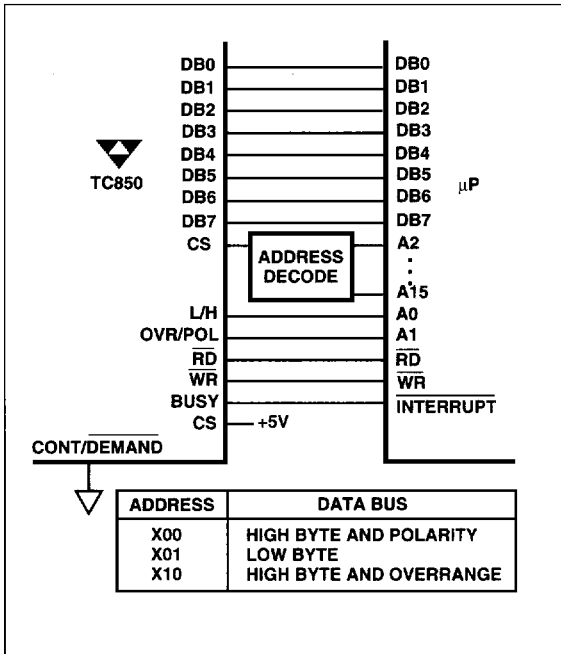
Figure 7. Interface to Typical \mu P Data Bus
