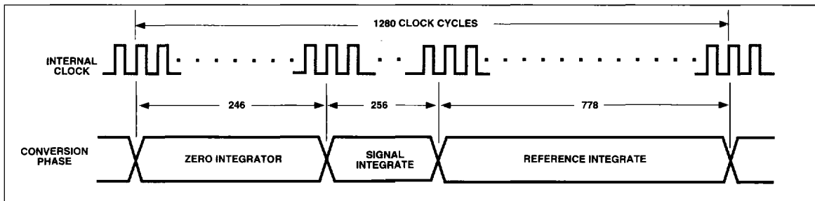
Figure 4. Conversion Timing
