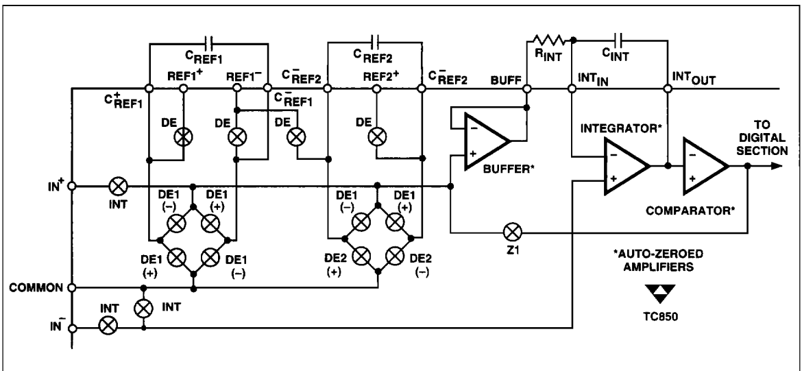
Figure 3. Analog Section Simplified Schematic
