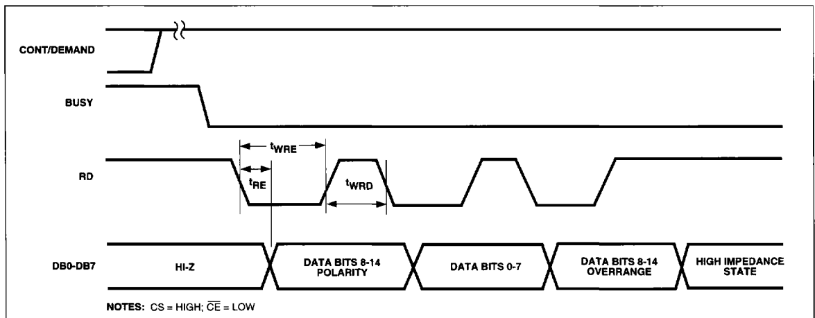
Figure 12. Bus Output Timing, Continuous Mode
