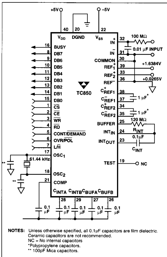
Figure 1. Standard Circuit Configuration
