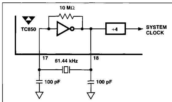
Figure 6. Crystal Oscillator Schematic
