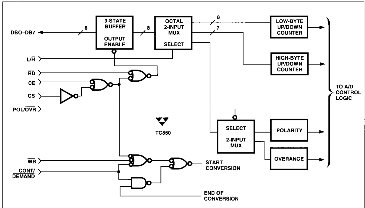
Figure 5. Bus Interface Simplified Schematic
