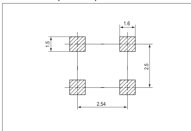
Dimensions(mm)
