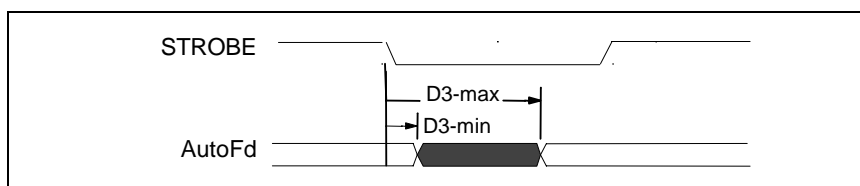
Figure 29 - Serial Interface Output Delay Timing
