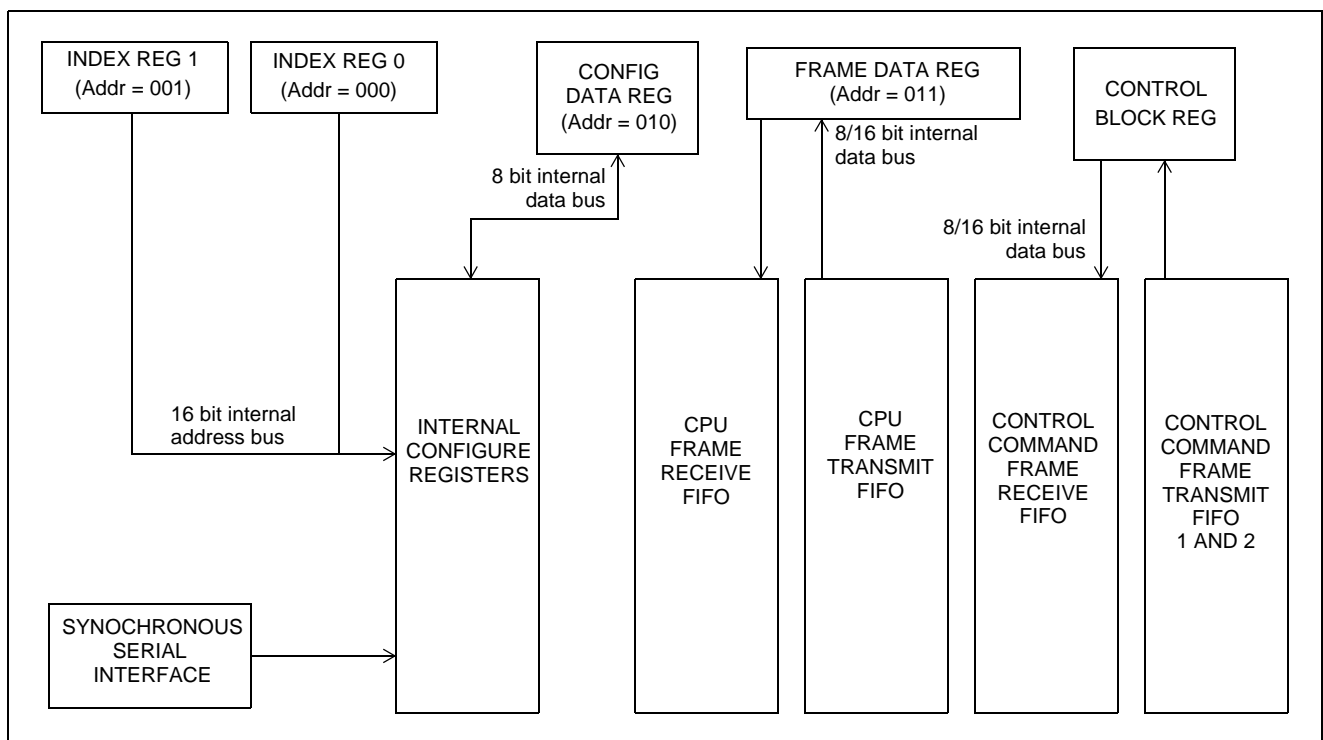
Figure 5 - Overview of the CPU Interface
