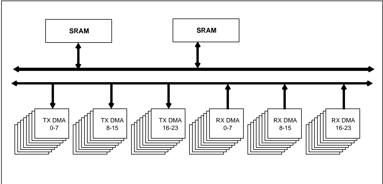
Figure 7 - SRAM Interface Block Diagram (DMAs for 10/100 Ports Only)
