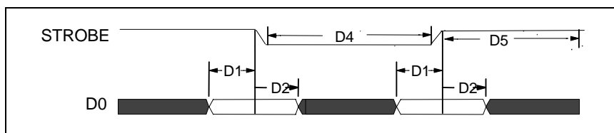
Figure 28 - Serial Interface Setup Timing
