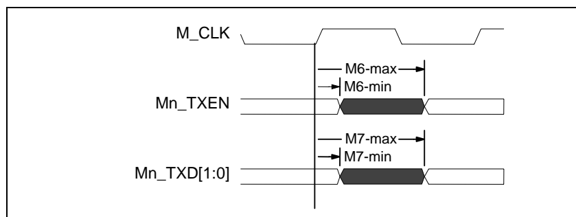
Figure 19 - AC Characteristics – Reduced Media Independent Interface
