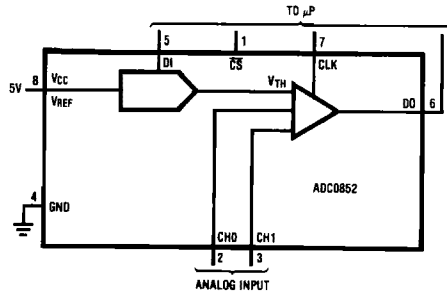
FIGURE 13. One Component Window Comparator
