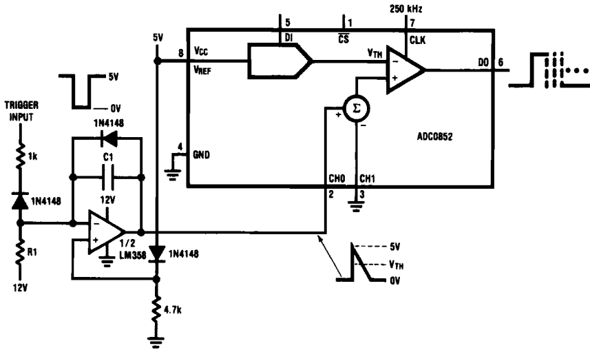
FIGURE 17. Pulse-Width Modulator
