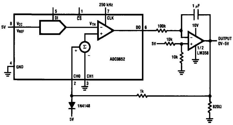
FIGURE 18. Serial Input 8-Bit DAC
