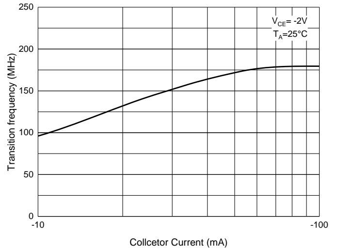
Fig. 4 - Transition frequency Characteristics
