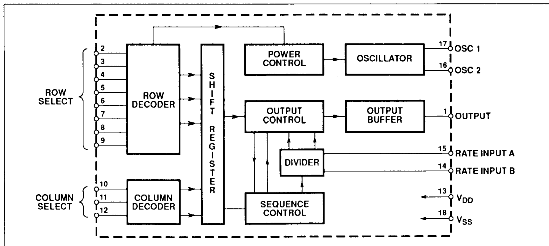
Fig.2 MV500 block diagram
