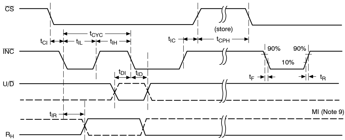
Figure 3. A.C. Timing
