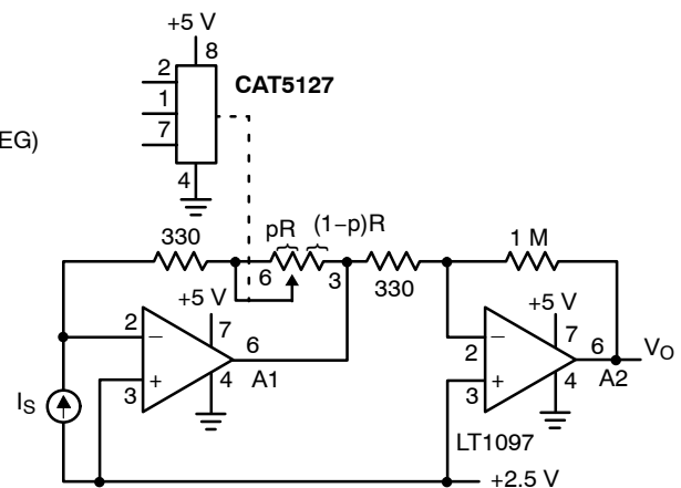
Figure 8. Programmable I to V Convertor
