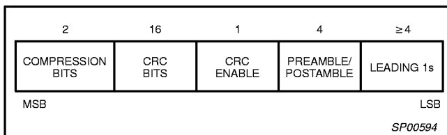
Figure 12. 27-bit Header
