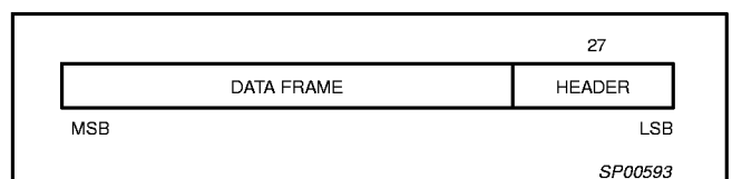
Figure 11. Data Packet
