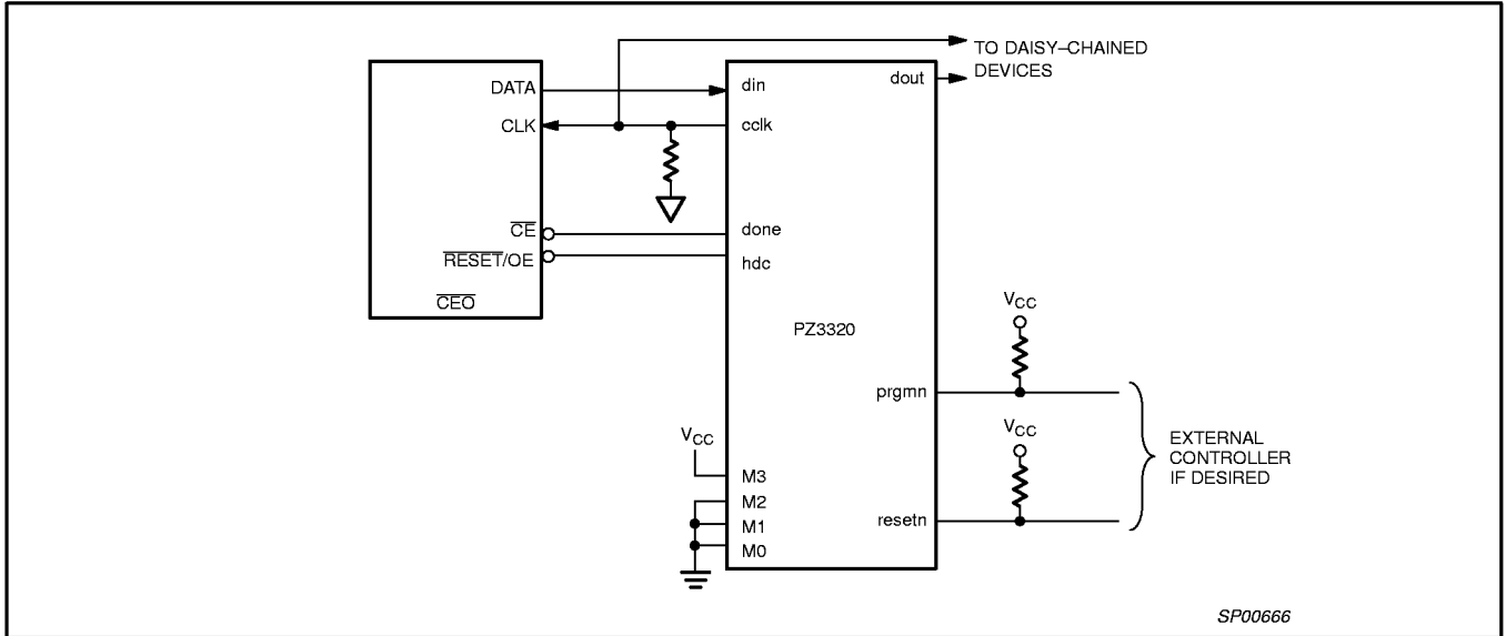
Figure 17. Master Serial Configuration
