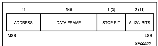
Figure 13. Standard Frame
