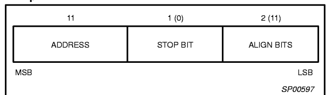
Figure 14. Compressed Frame
