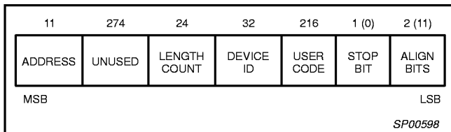
Figure 15. User code Frame
