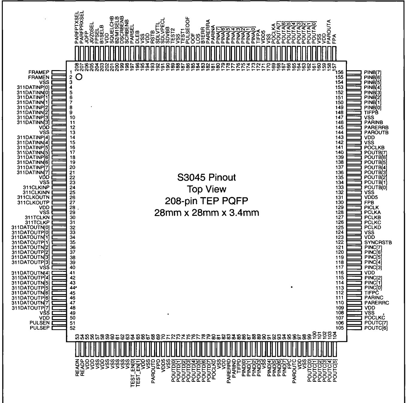
Figure 14. S3045 Pinout
