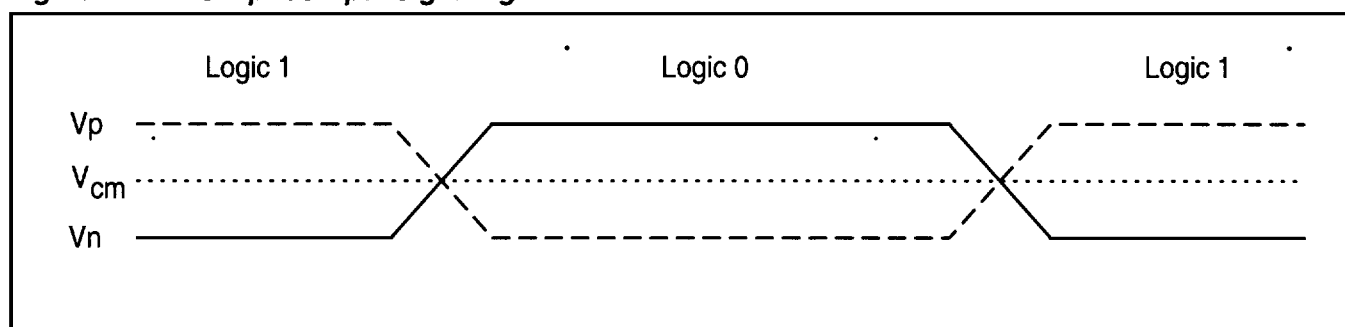
Figure 22. LVDS Input/Output Signaling
