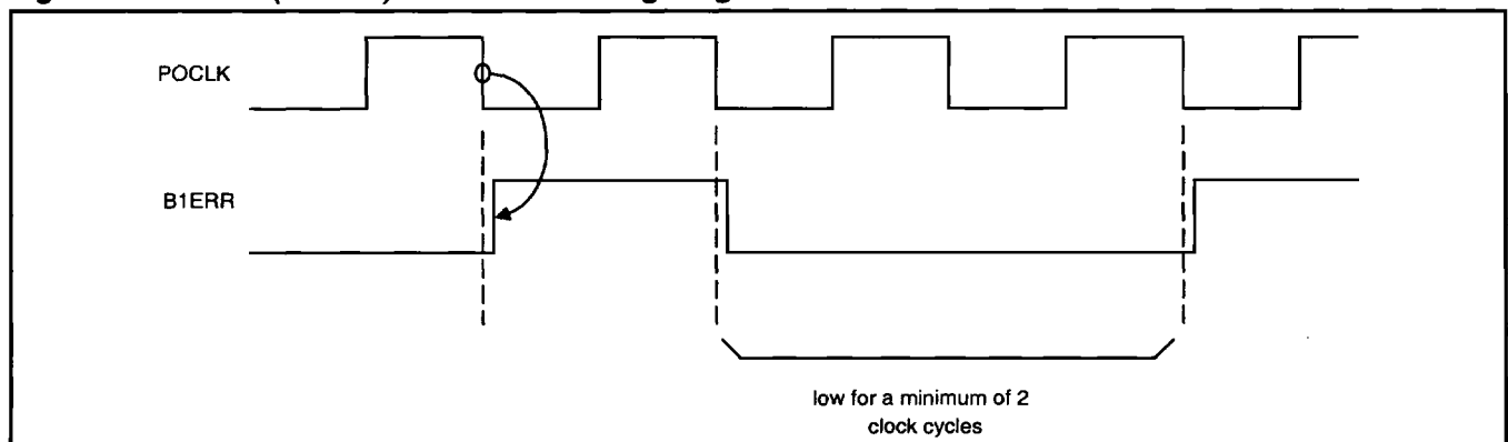
Figure 4. B1 Error (B1ERR) Functional Timing Diagram
