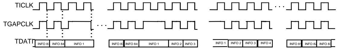
Figure 42: Framer Mode DS3 Transmit Input Stream With TGAPCLK
