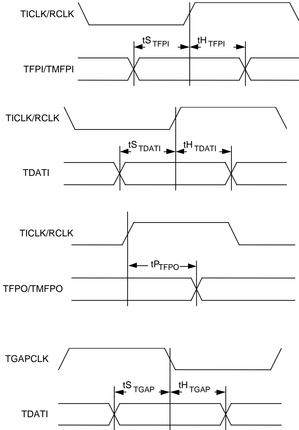
Figure 57: DS3 Transmit Interface Timing
