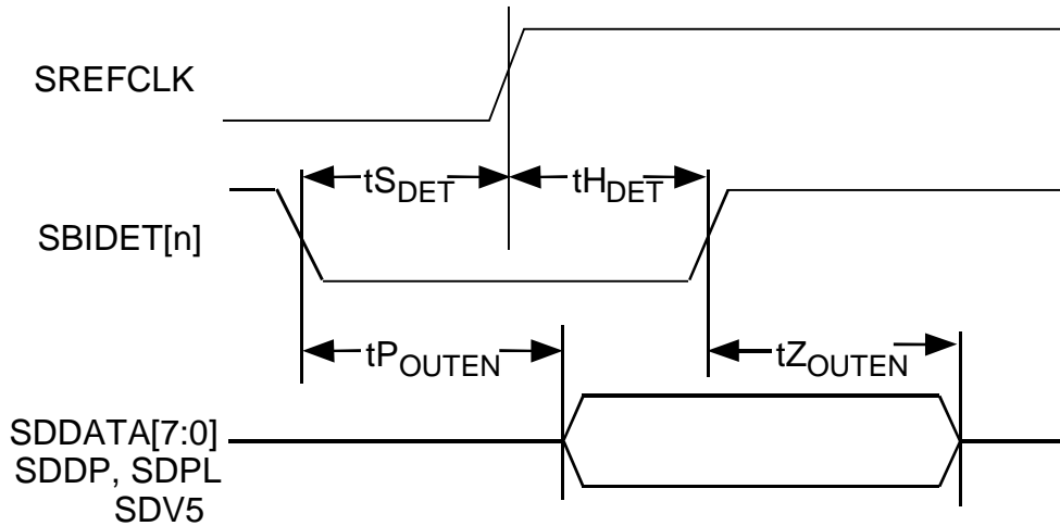
Figure 64: SBI DROP BUS Collision Avoidance Timing
