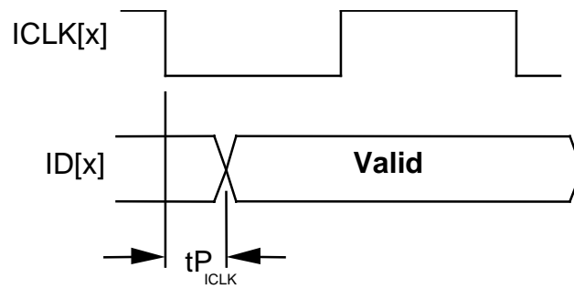
Figure 67: Ingress Interface Timing - Clock Master: Clear Channel Mode
