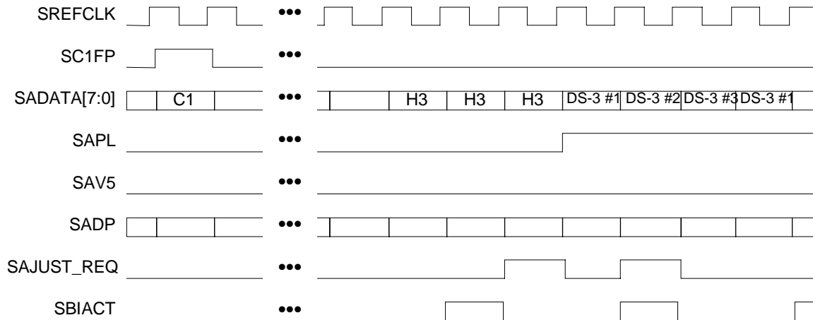
Figure 53: SBI ADD Bus Adjustment Request Functional Timing
