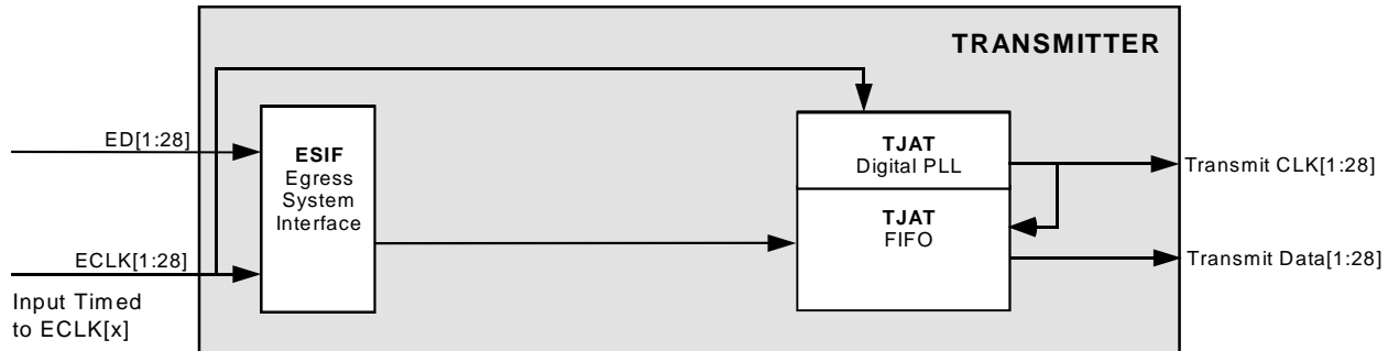
Figure 15 - Clock Slave: Clear Channel
