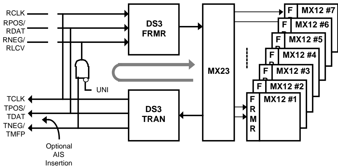
Figure 25: DS3 Diagnostic Loopback Diagram
