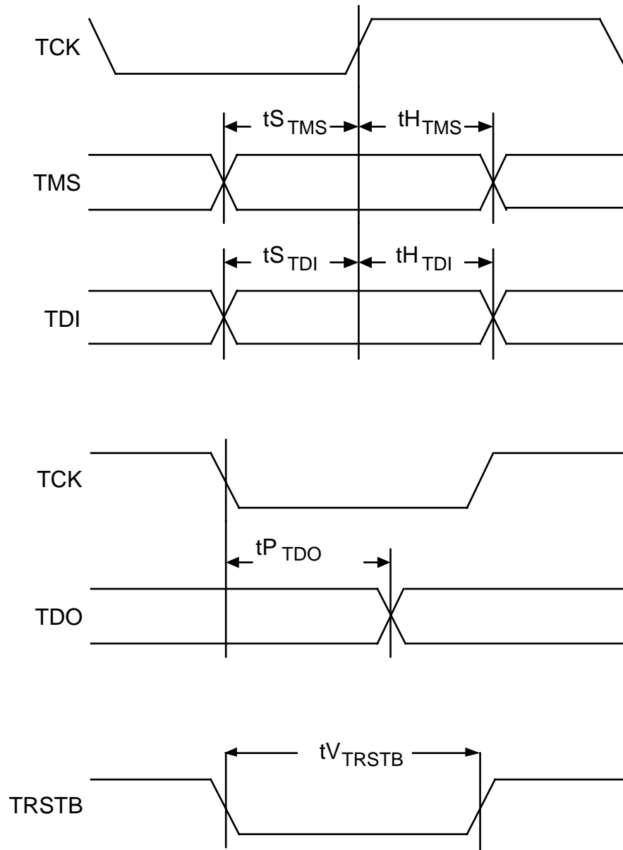
Figure 70: JTAG Port Interface Timing
