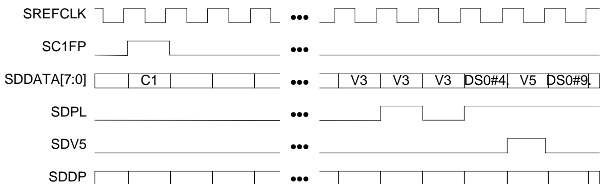
Figure 51: SBI DROP Bus T1/E1 Functional Timing
