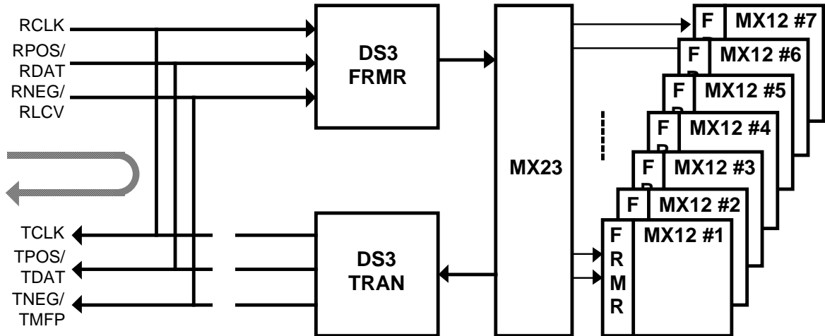
Figure 26: DS3 Line Loopback Diagram
