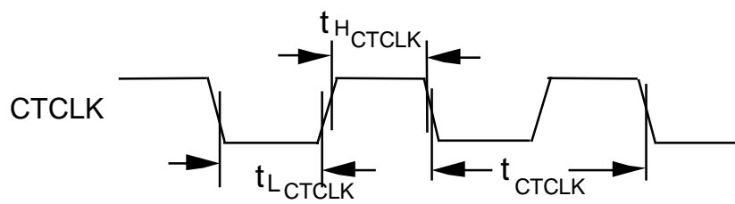
Figure 68: Transmit Line Interface Timing
