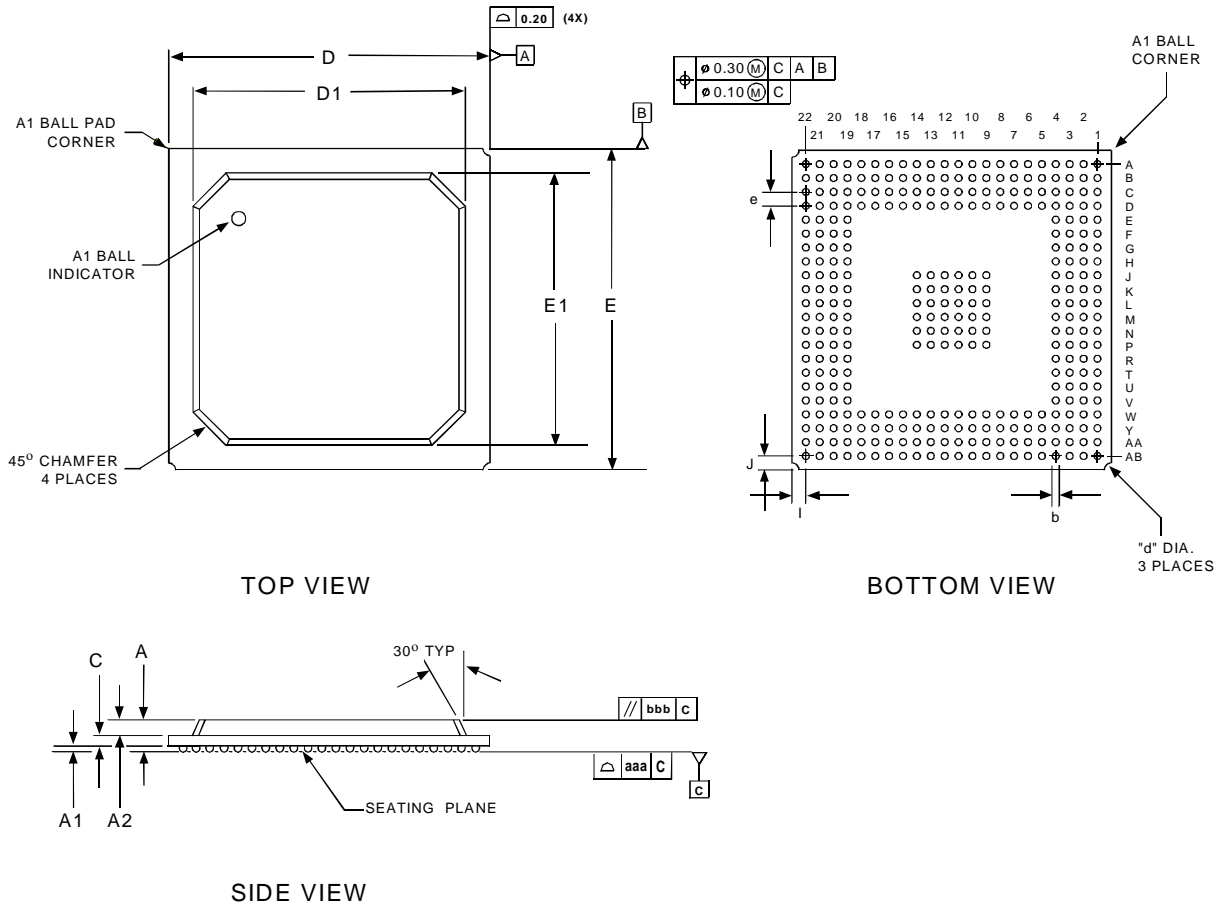
Figure 71: 324 Pin PBGA 23x23mm Body
