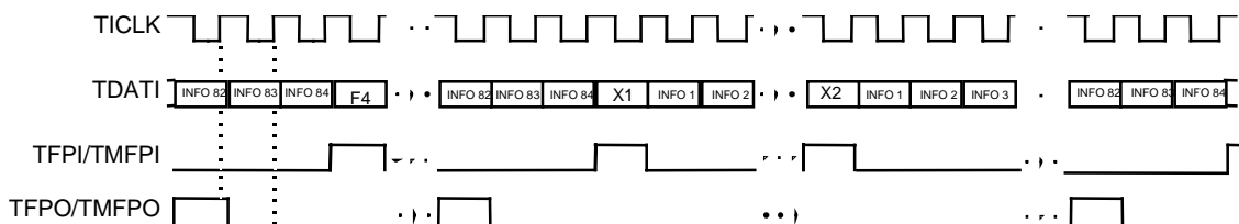
Figure 41: Framers Mode DS3 Transmit Input Stream
