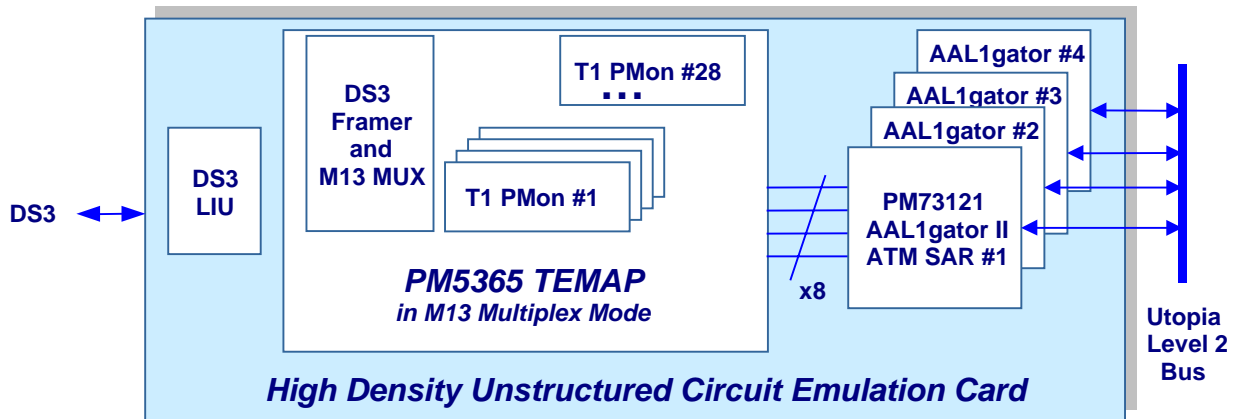
Figure 1 - DS3 Multiplexing Application
