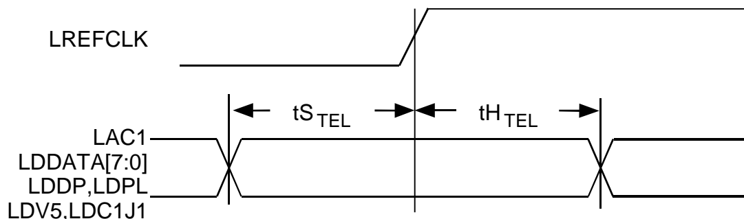
Figure 59: Line Side Telecom BUS InputTiming
