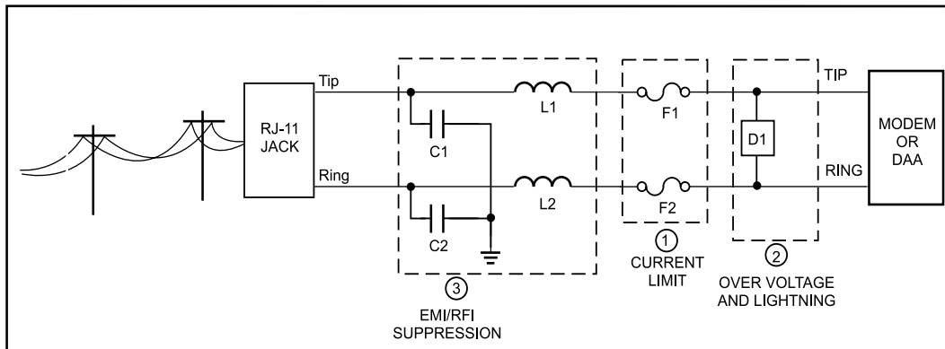
Figure 6. Telephone Interfaces
