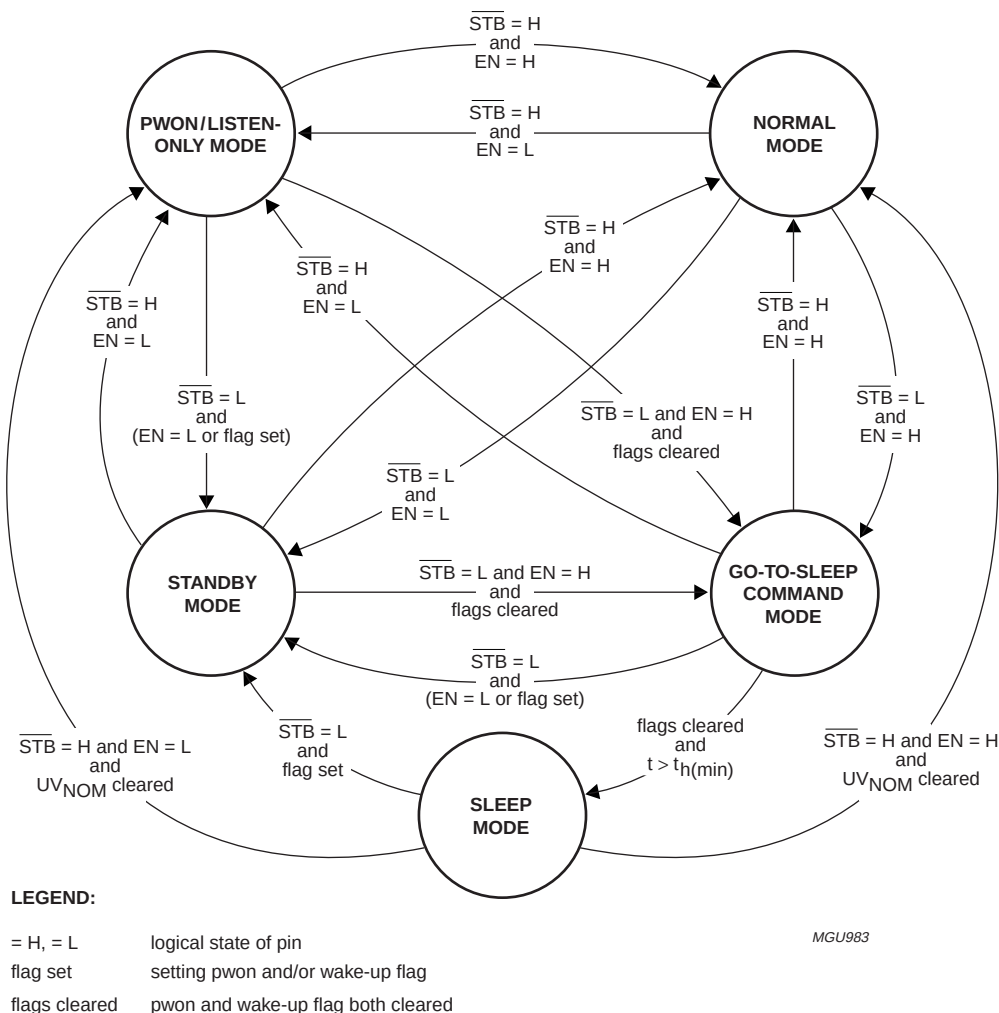
Fig.3 Mode transitions when V_{CC} , V_{IO} and V_{BAT} are present.
