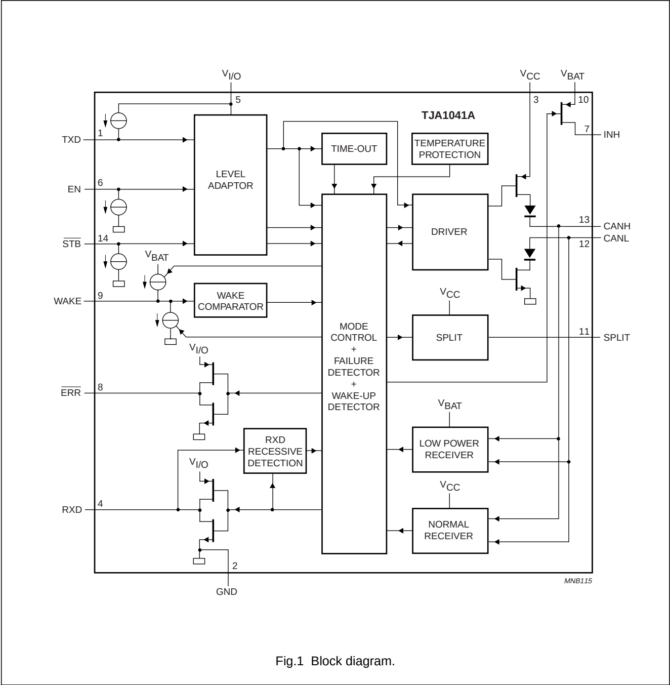
BLOCK DIAGRAM
