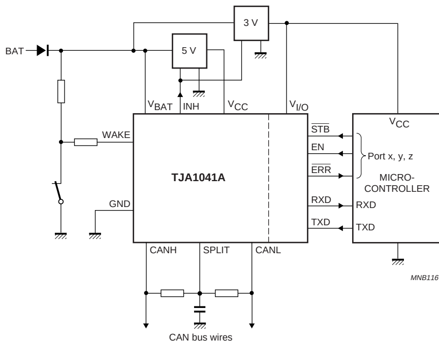
Fig.4 Typical application with 3 V microcontroller.
