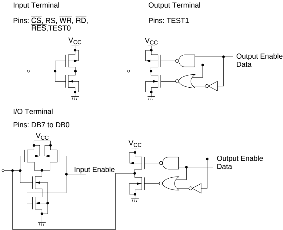
Figure 39 Terminal Configuration
