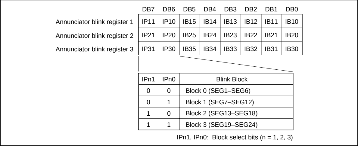
Figure 18 Annunciator Blink Registers
