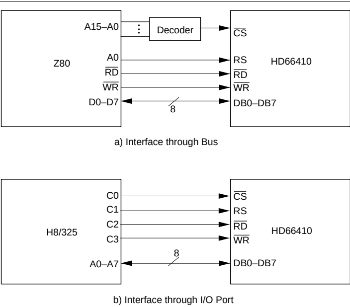
Figure 2 8-Bit MPU Interface Examples
