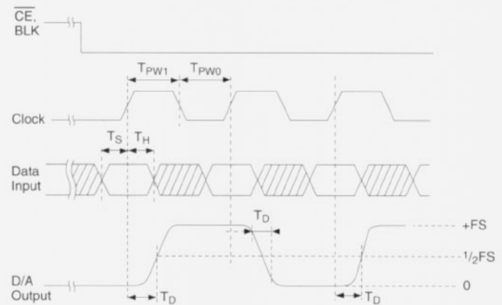
Timing Diagram
