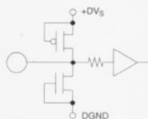
Digital input, BLK, CE and CLK inputs
