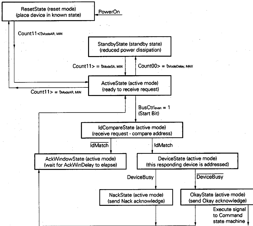
Figure 6-1. Frame State Machine - State Diagram
