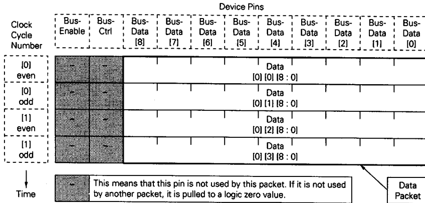
Figure 5-3. Data Packet Format (Register Space)
