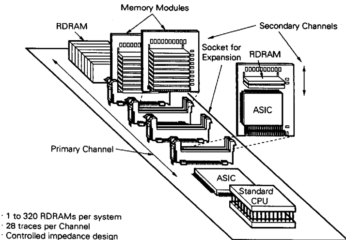
Figure 2-2. A Rambus System Example
