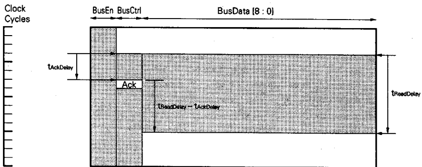
Figure 7-1. Read Transaction
