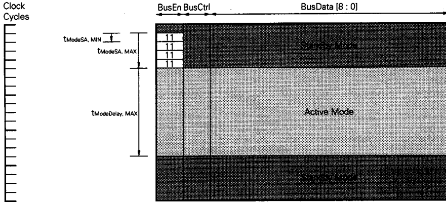
Figure 6-2. Basic ActiveMode/StandbyMode Transitions
