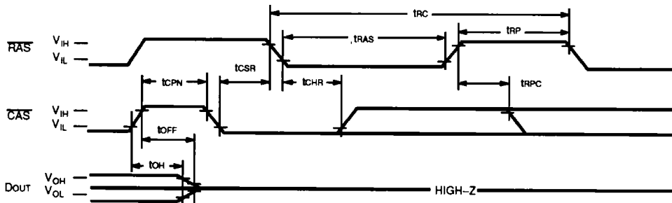
Fig. 11 - \overline{\text{CAS}} -BEFORE- \overline{\text{RAS}} REFRESH CYCLE
