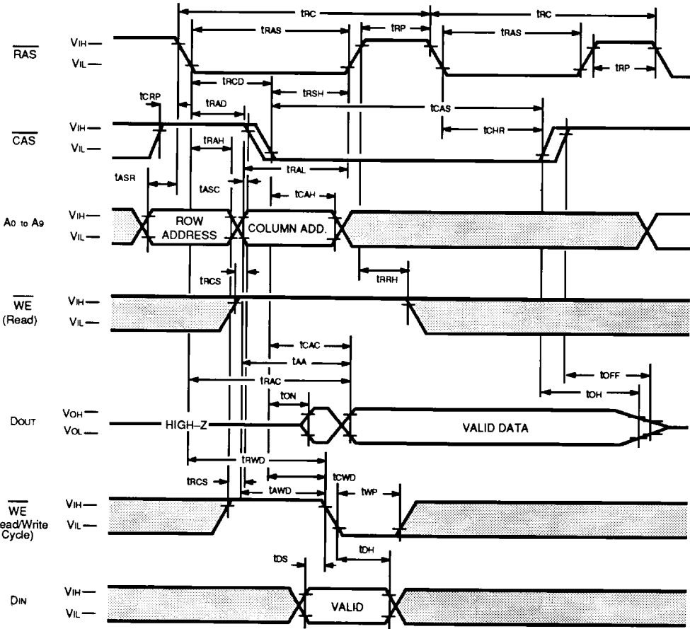
Fig. 13 - HIDDEN REFRESH CYCLE
