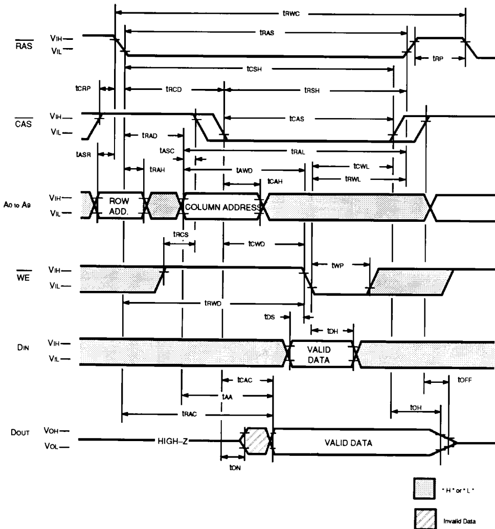
Fig. 6 – READ WRITE/READ-MODIFY-WRITE CYCLE
