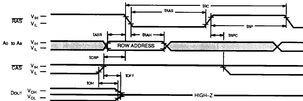
Fig. 10 - \overline{\text{RAS}} -ONLY REFRESH CYCLE
