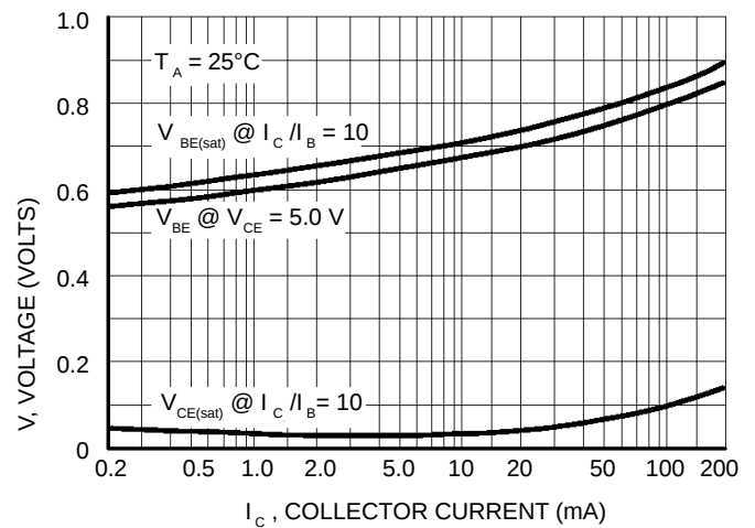
Figure 8. "On" Voltage
