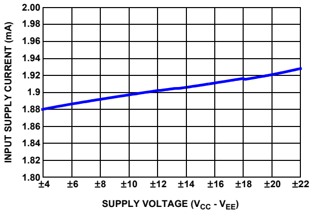
FIGURE 26. I_{CC} vs SUPPLY VOLTAGE ( V_{CC} - V_{EE} )
