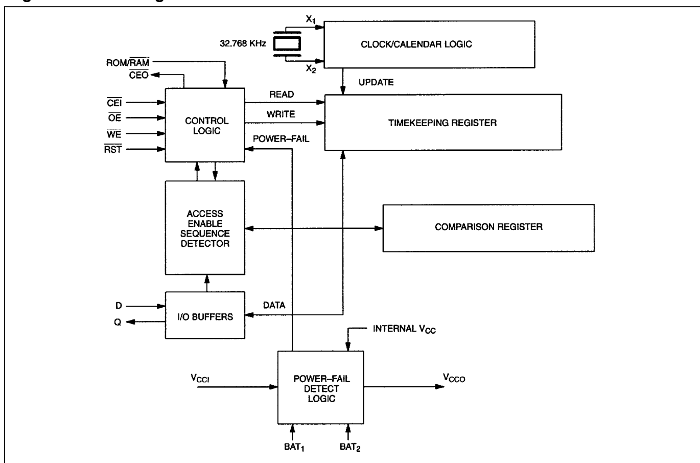
Figure 1. Block Diagram
