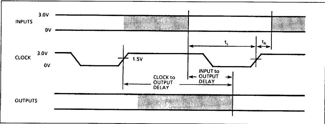
Figure 30: AC Timings
