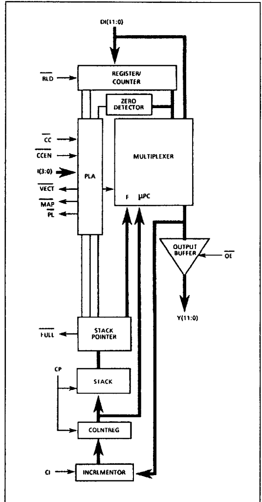
Figure 1: Block Diagram
