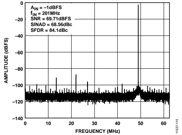
Figure 15. Single-Tone 32k FFT with f_{IN} = 201 MHz; f_{SAMPLE} = 125 MSPS
