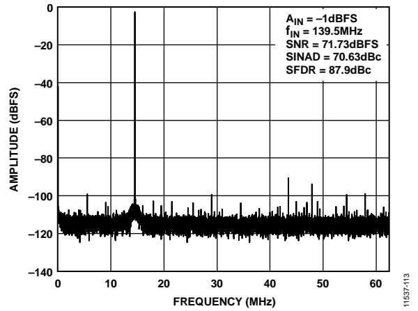
Figure 14. Single-Tone 32k FFT with f_{IN} = 139.5 MHz; f_{SAMPLE} = 125 MSPS
