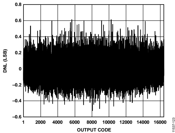
Figure 23. DNL; f_{IN} = 9.7 \text{ MHz} , f_{SAMPLE} = 125 \text{ MSPS}
