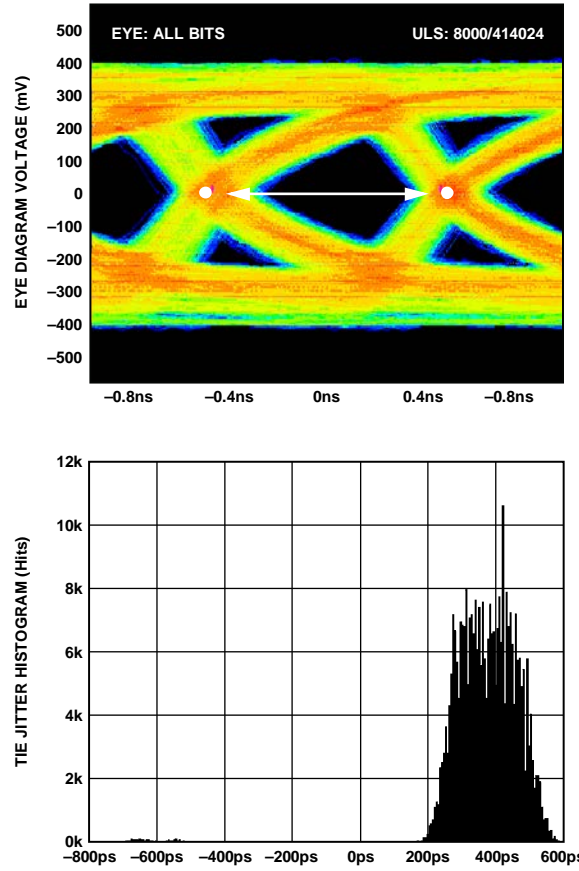
Figure 52. Data Eye for LVDS Outputs in ANSI-644 Mode with Trace Lengths of Greater Than 24 Inches on Standard FR-4 Material, External 100Ω Far End Termination Only
