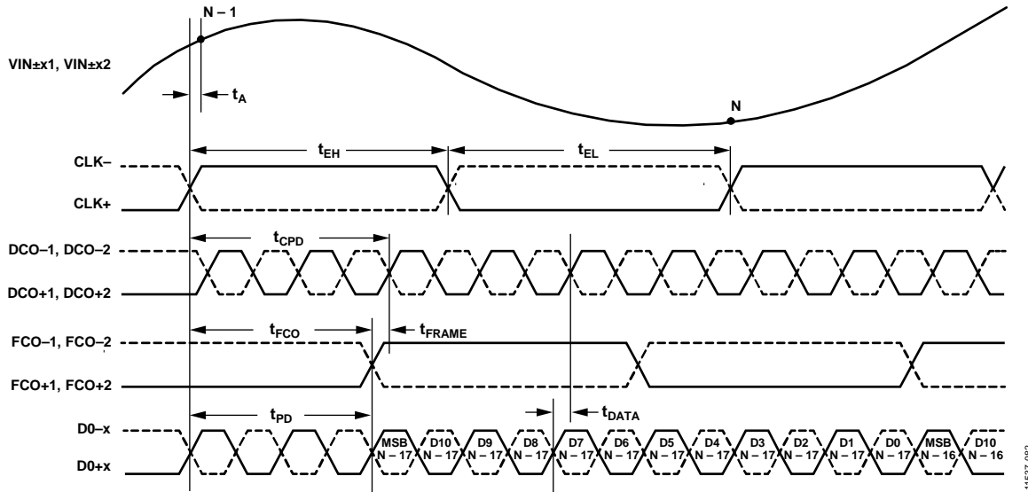
Figure 8. Wordwise DDR, One-Lane, 1x Frame, 12-Bit Output Mode
