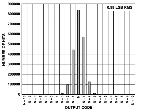
Figure 24. Input Referred Noise Histogram; f_{SAMPLE} = 125 \text{ MSPS}
