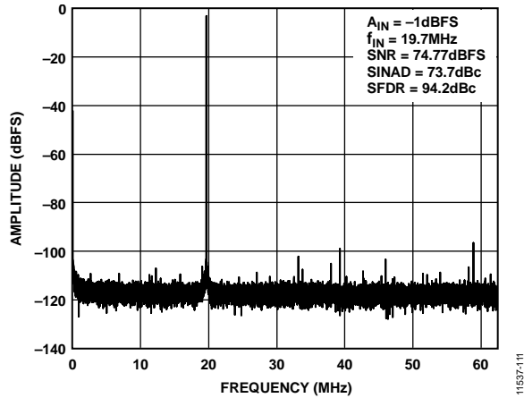
Figure 12. Single-Tone 32k FFT with f_{IN} = 19.7 MHz; f_{SAMPLE} = 125 MSPS
