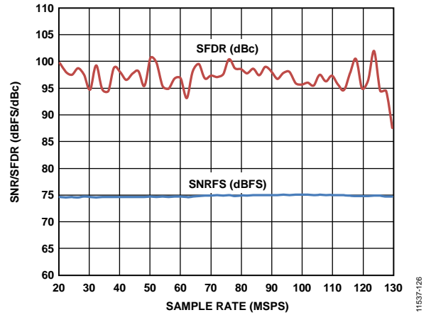
Figure 25. SNR/SFDR vs. Sample Rate; f_{IN} = 9.7 \text{ MHz} , f_{SAMPLE} = 125 \text{ MSPS}
