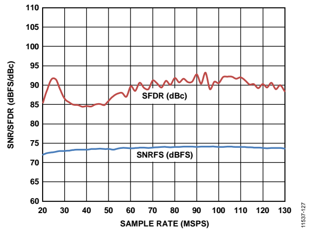
Figure 26. SNR/SFDR vs. Sample Rate; f_{IN} = 70 \text{ MHz} , f_{SAMPLE} = 125 \text{ MSPS}
