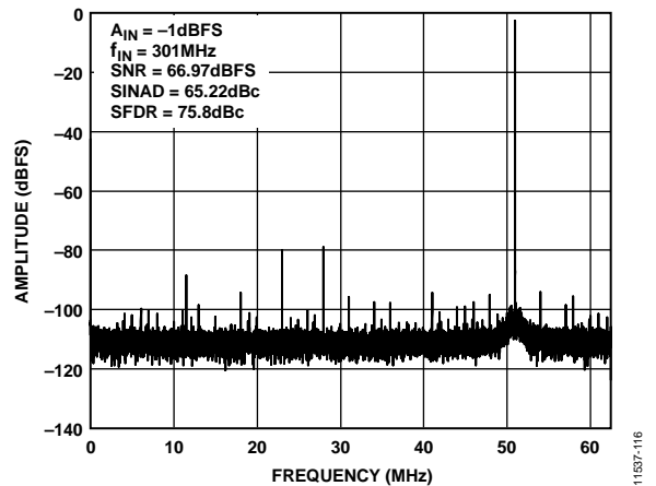
Figure 16. Single-Tone 32k FFT with f_{IN} = 301 MHz; f_{SAMPLE} = 125 MSPS
