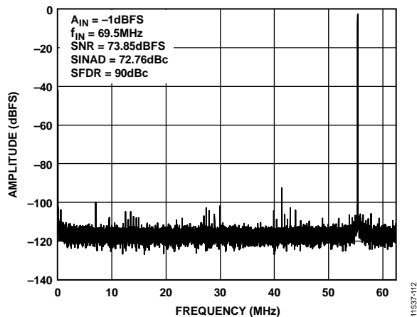
Figure 13. Single-Tone 32k FFT with f_{IN} = 69.5 MHz; f_{SAMPLE} = 125 MSPS
