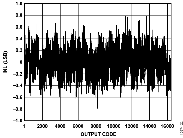
Figure 22. INL; f_{IN} = 9.7 \text{ MHz} , f_{SAMPLE} = 125 \text{ MSPS}
