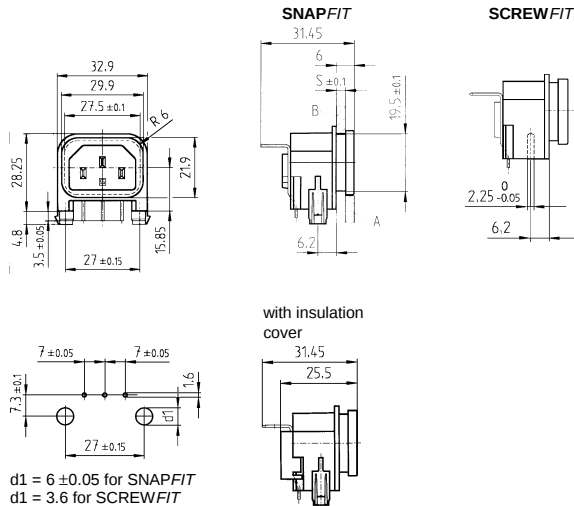
rear panel mounting
