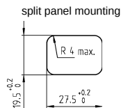
split panel mounting
