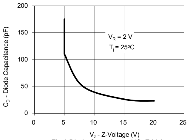
Fig.6 Diode Capacitance VS. Z-Voltage
