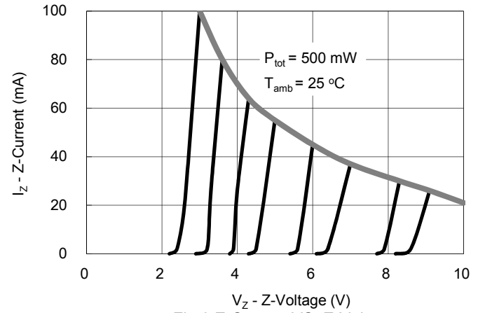
Fig.8 Z-Current VS. Z-Voltage
