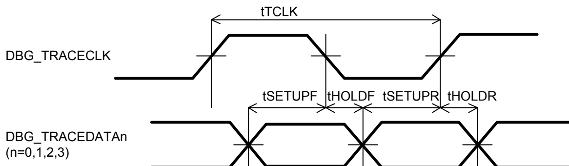
Figure 6-15 Trace Interface Timing
