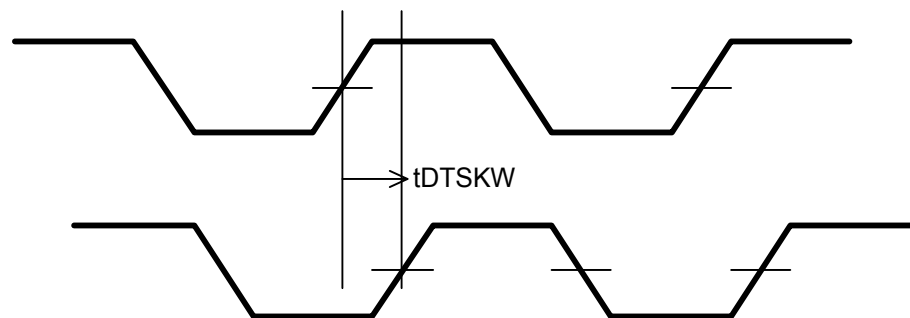
Figure 6-21 EBIF Timing Diagram on Data Skew
