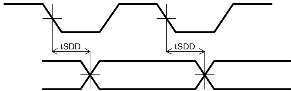
Figure 6-26 eMMC/SD Card/SDIO Interface Timing in High Speed SDR (eMMC)/High Speed (SD Card, SDIO) Mode
