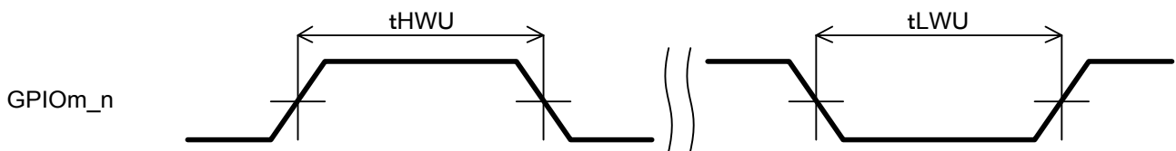
Figure 6-11 GPIO Input Timing
