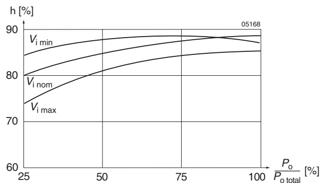
Fig. 13 Efficiency versus input voltage and load. Typical values 110IMY15-12-12-8
