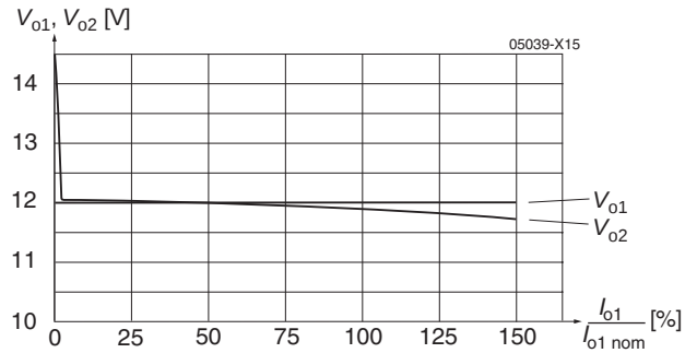
Fig. 12 Flexible load distribution on double outputs models with option R (110IMY15-12-12-8R): Load variation from 0 to 150% of P_{o1\text{ nom}} on output 1. Output 2 loaded with 50% of P_{o2\text{ nom}} .
