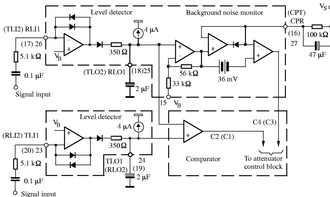
Figure 5. Level detectors
