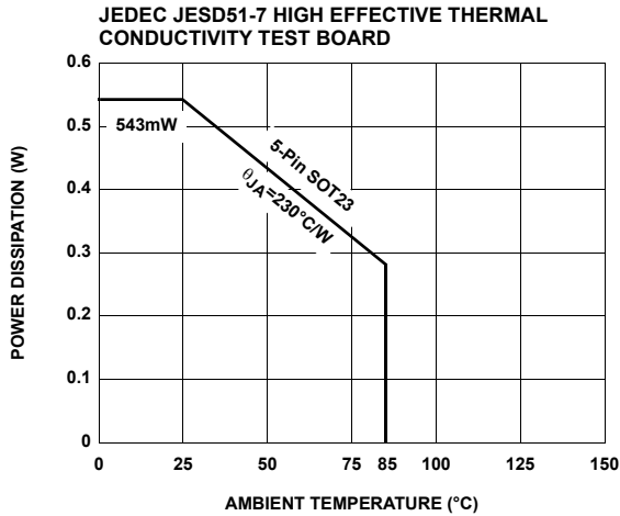
FIGURE 5. PACKAGE POWER DISSIPATION VS AMBIENT TEMPERATURE
