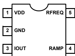
EL6206 (5-PIN SOT23) TOP VIEW
