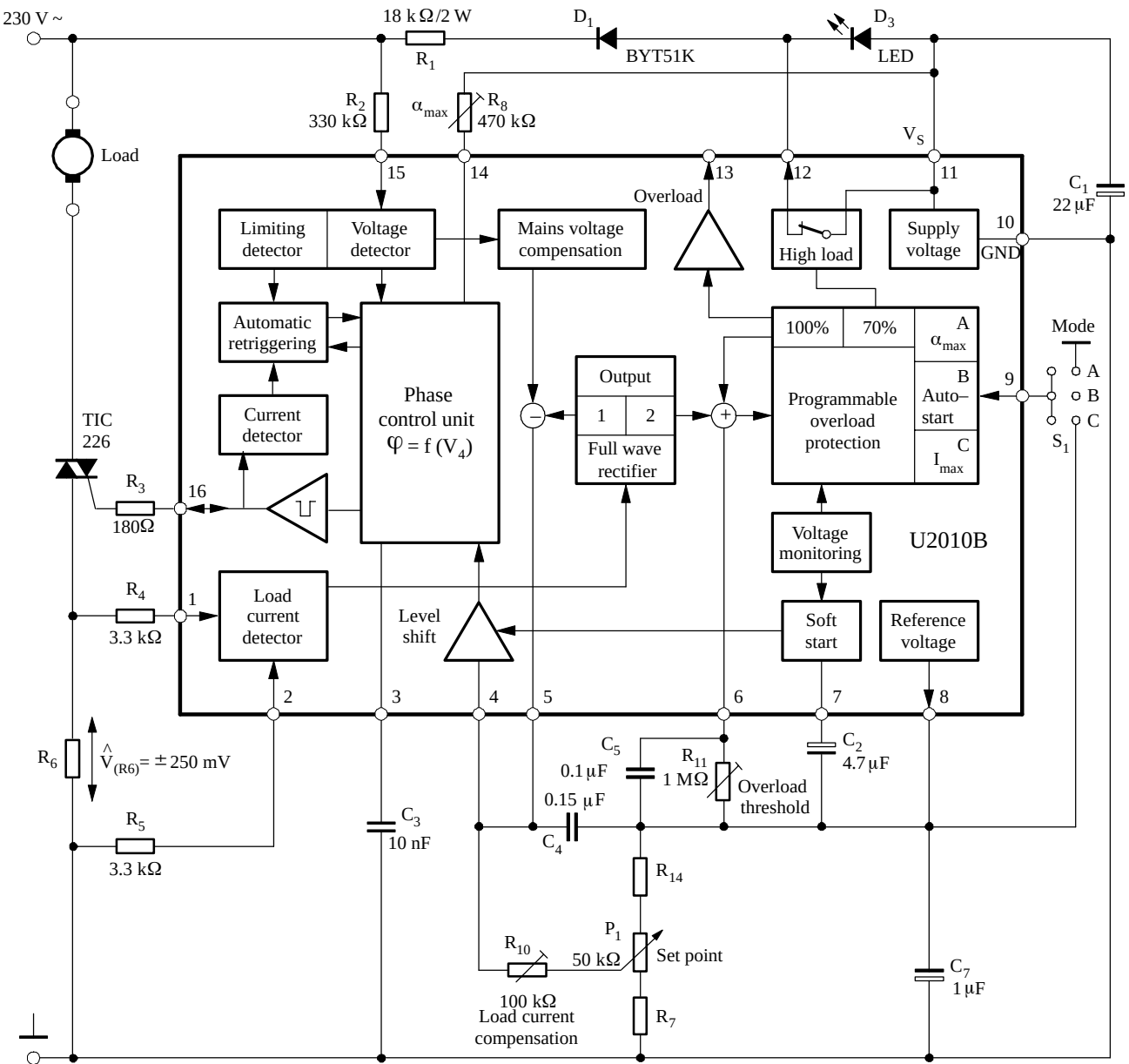
Figure 2. Block diagram with external circuit
