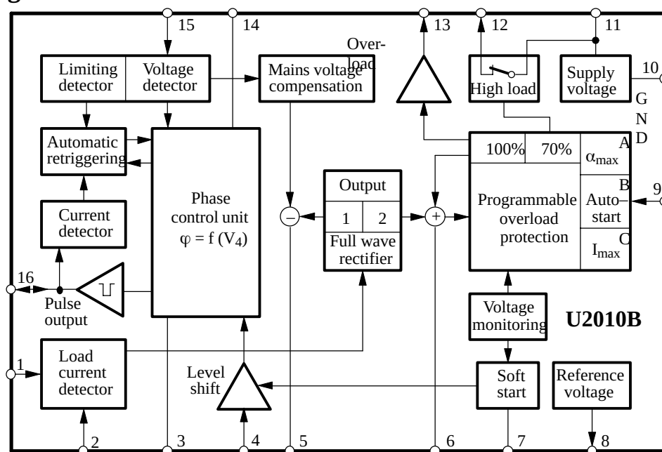
Figure 1. Block diagram
