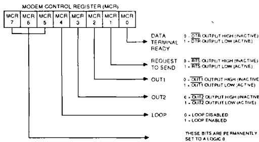
Figure 5 : MODEM CONTROL REGISTER
