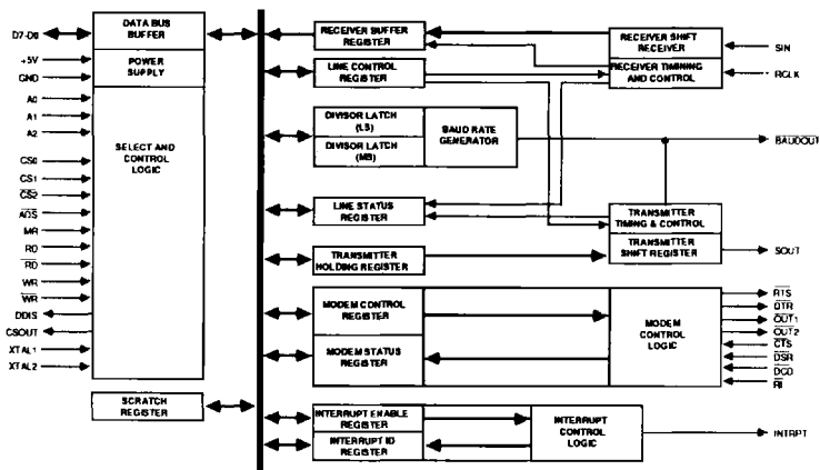
Figure 1 : BLOCK DIAGRAM OF KS82C50A
