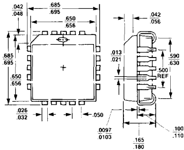
Figure 9 : PLCC PACKAGING
