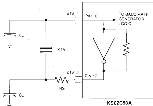
Figure 7 : CRYSTAL OSCILLATOR CIRCUIT
