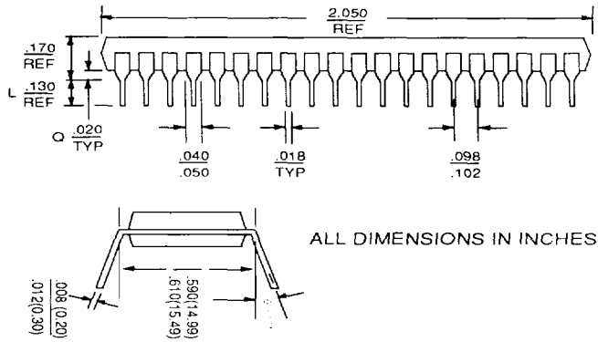
Figure 8 : PLASTIC PACKAGING
