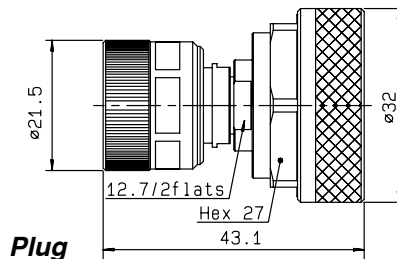
Plug
