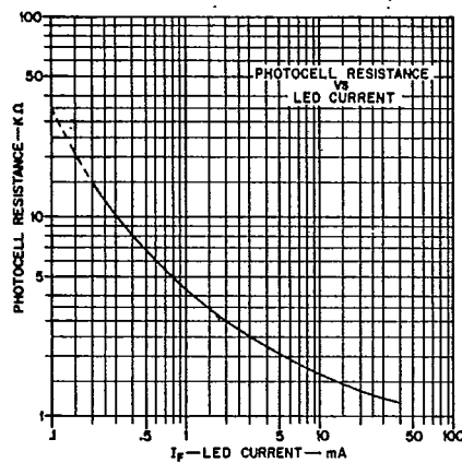
RESISTANCE vs. LED CURRENT
