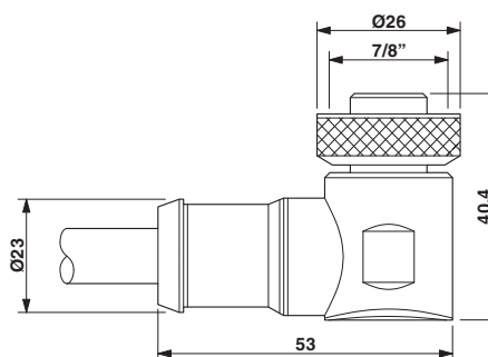
Dimensional drawing
