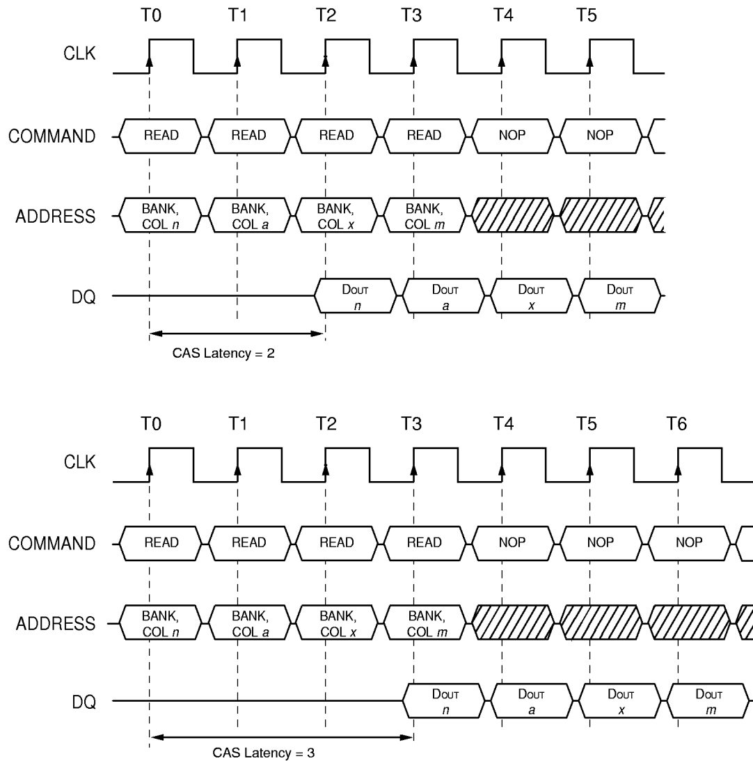
Figure 8 RANDOM READ ACCESSES WITHIN A PAGE
