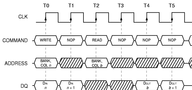
Figure 16 RANDOM WRITE CYCLES WITHIN A PAGE
