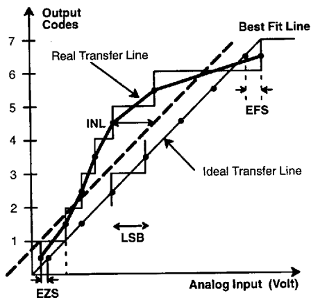
Figure 4. INL Error Calculation
