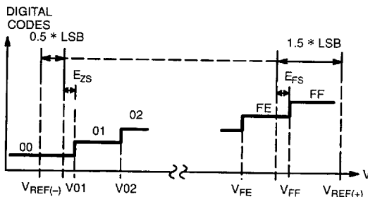
Figure 8. Real A/D Transfer Curve
