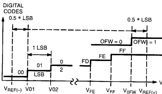
Figure 7. Ideal A/D Transfer Function
