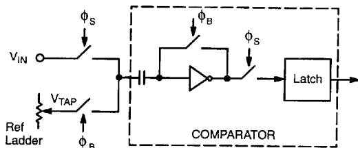
Figure 6. MP7684A Comparator
