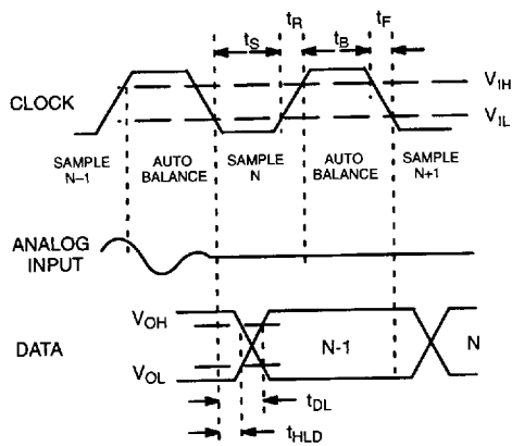
Figure 1. MP7684 Timing Diagram
