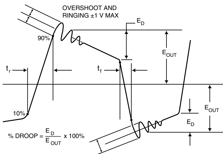
FIGURE 1. WAVEFORM INTEGRITY
