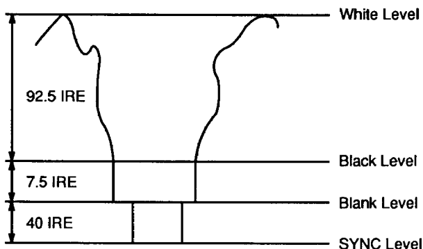
Figure 2. Composite Video Output Signals
