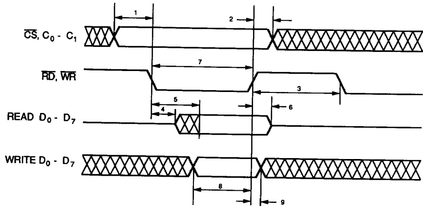
MPU Read/Write Timing
