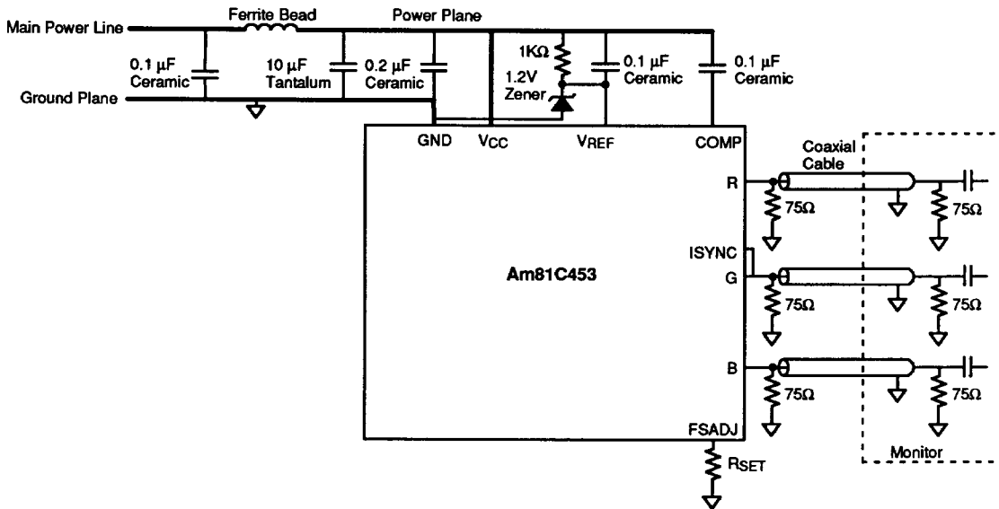
Figure 1. Am81C453 Typical Circuit Connection
