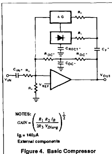
Figure 4. Basic Compressor
