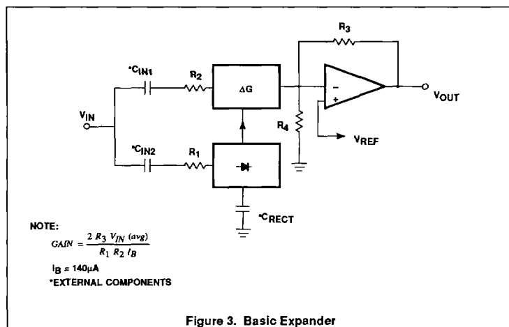
Figure 3. Basic Expander
