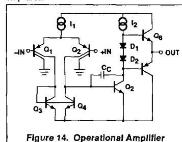
Figure 14. Operational Amplifier
