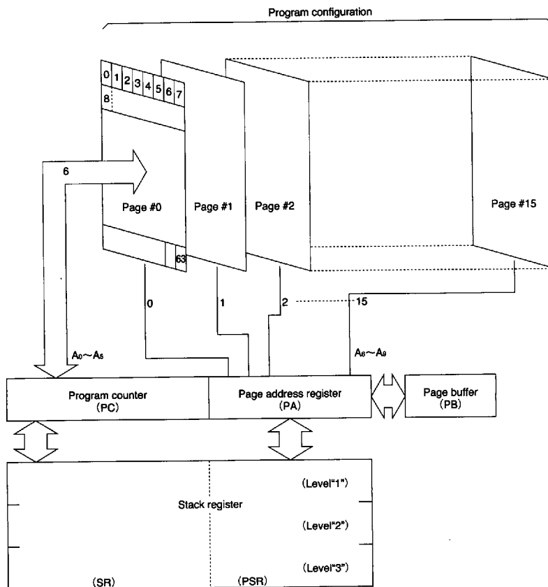
Fig. 9 Program memory configuration
