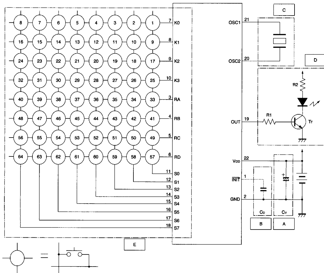
Fig. 8 Application circuit example (64-key remote control unit)
