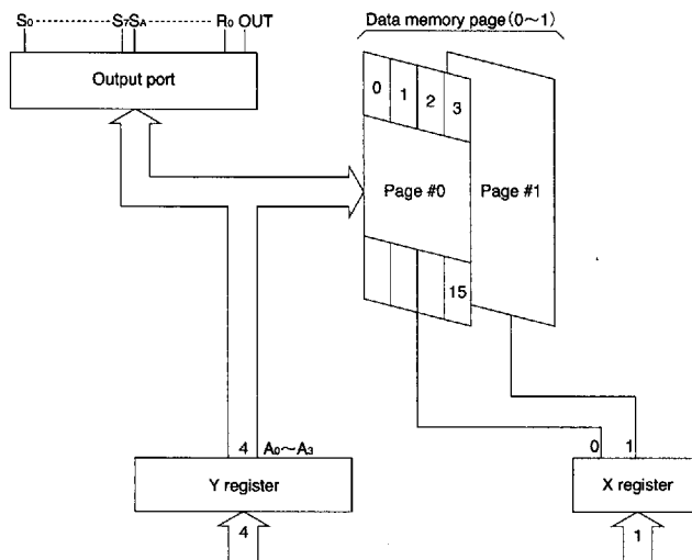
Fig. 10 Data memory configuration
