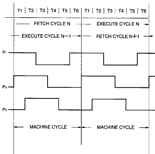
Fig. 11 Basic timing chart
