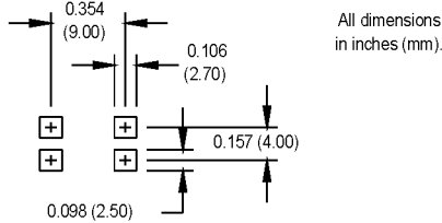
SUGGESTED SOLDER PAD LAYOUT
