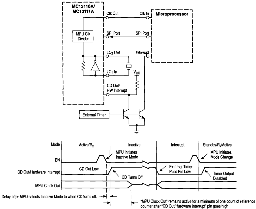
Figure 120. Power Saving Application – Option 2 (MC13110A/MC13111A Only)
