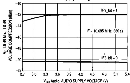
Figure 21. First Mixer Compression versus Supply Voltage
