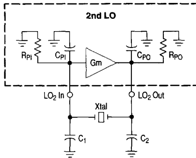
Figure 40. Second Local Oscillator Input and Output Impedance
