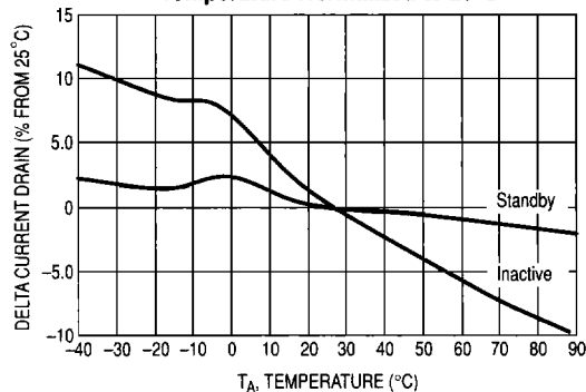
Figure 7. Current versus Temperature Normalized to 25°C
