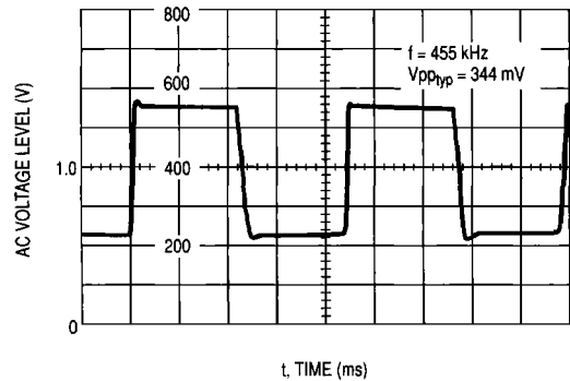
Figure 53. Typical Limiter Output Waveform with Quadrature Coil
