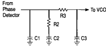
Figure 100. Loop Filter with Additional Integrating Element
