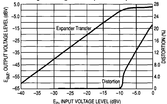
Figure 76. R x Audio Expander Response
