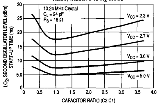
Figure 43. Start-Up Time versus Capacitor Ratio, Inactive to R_x Mode
