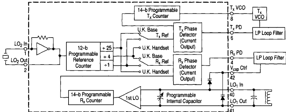
Figure 95. Dual PLL Simplified Block Diagram
