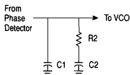
Figure 97. Loop Filter with Additional Integrating Element
