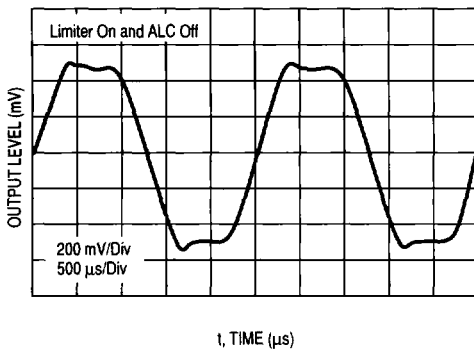
Figure 92. T x Output Audio Response
