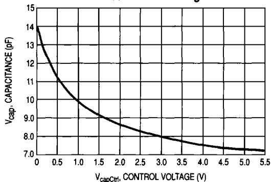
Figure 33. First LO Varicap Capacitance versus Control Voltage
