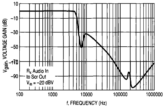
Figure 71. R x Audio Wideband Frequency Response
