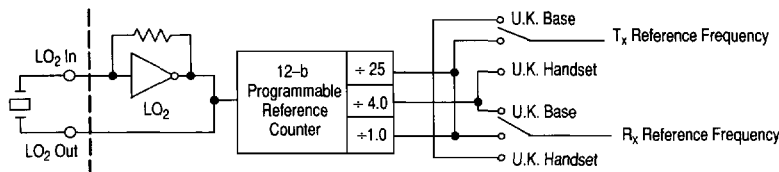
Figure 113. Reference Counter Register Programming Mode
