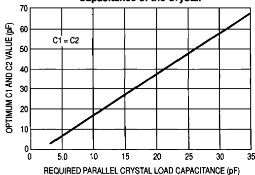
Figure 47. Optimum Value for C1 and C2 versus Equivalent Required Parallel Capacitance of the Crystal
