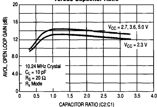
Figure 45. Maximum Open Loop Gain versus Capacitor Ratio
