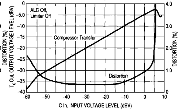
Figure 89. T x Audio Compressor Response
