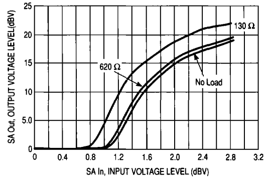
Figure 80. R x Audio Speaker Amplifier Distortion
