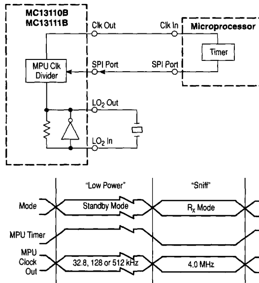
Figure 119. Power Saving Application – Option 1
