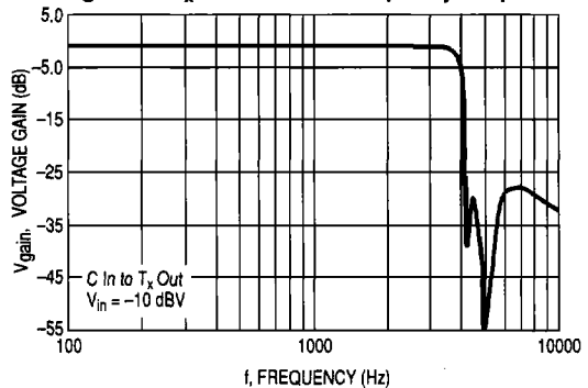
Figure 83. T x Audio Inband Frequency Response
