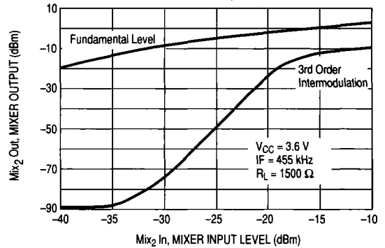
Figure 29. Second Mixer Output Level and Intermodulation, IP3_bit = 1
