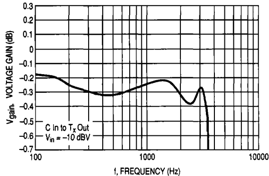
Figure 84. T x Audio Ripple Response
