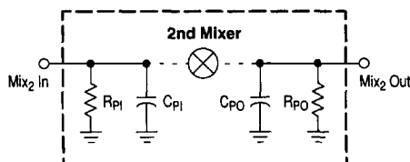
Figure 24. Second Mixer Input and Output Impedances
