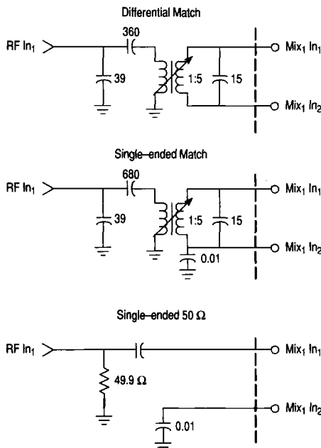
Figure 60. Matching Input Networks
