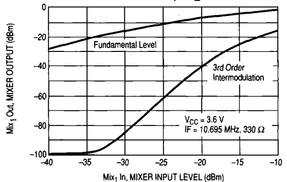
Figure 20. First Mixer Output Level and Intermodulation, IP3_bit = 1
