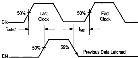
Figure 106. Enable Timing Requirement
