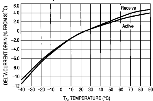
Figure 8. Current versus Temperature Normalized to 25°C
