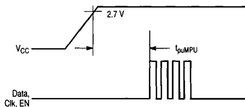
Figure 108. Microprocessor Serial Interface Power-Up Delay
