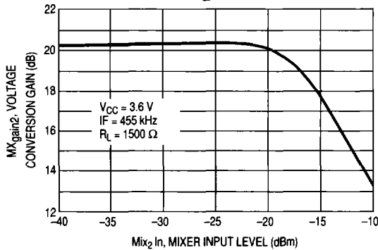
Figure 26. Second Mixer Conversion Gain, IP3_bit = 0
