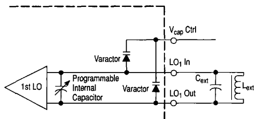
Figure 32. First Local Oscillator Schematic
