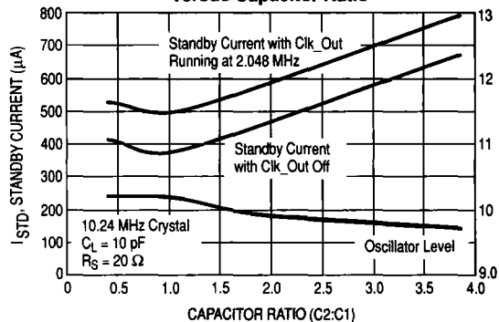
Figure 44. Second LO Current Consumption versus Capacitor Ratio
