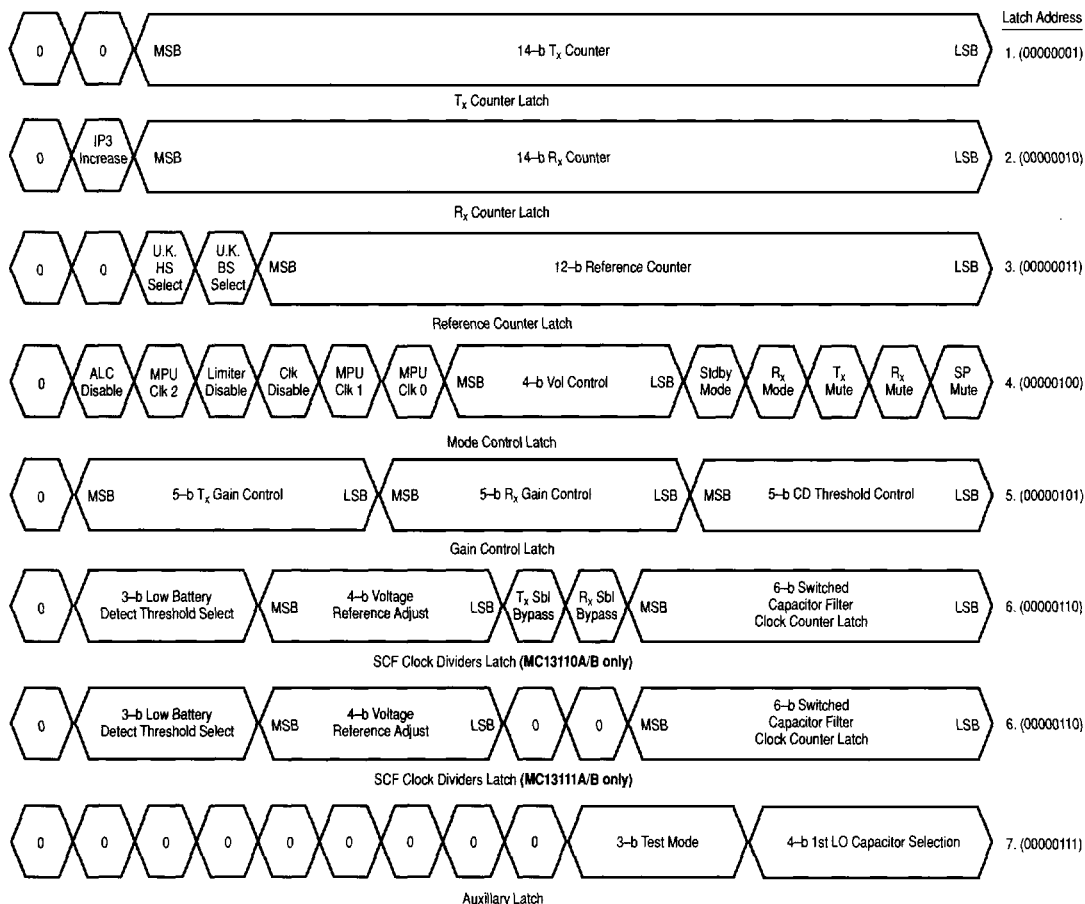
Figure 109. Microprocessor Interface Data Latch Registers
