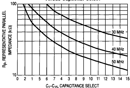
Figure 35. Representative Parallel Impedance versus Capacitor Select
