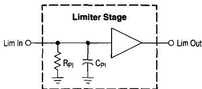
Figure 49. Limiter Input Impedance
