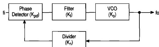
Figure 96. PLL Model
