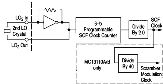
Figure 132. SCF Clock Divider Circuit
