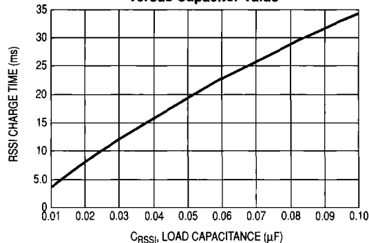
Figure 59. RSSI Charge Time versus Capacitor Value
