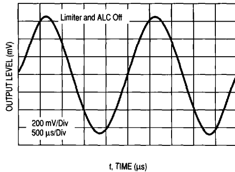
Figure 91. T x Output Audio Response
