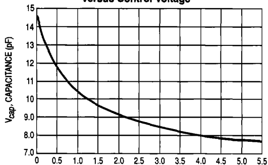
Figure 99. Varicap Capacitance versus Control Voltage
