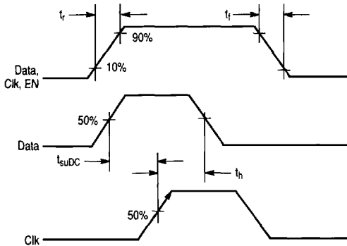
Figure 105. Data and Clock Timing Requirement
