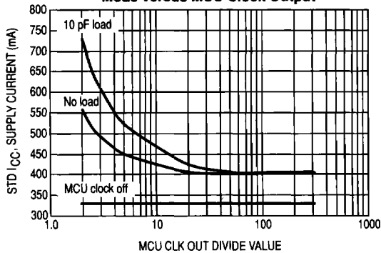
Figure 11. Current Standby Mode versus MCU Clock Output
