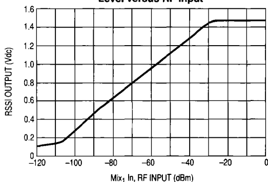
Figure 56. Typical RSSI Voltage Level versus RF Input
