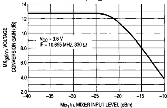
Figure 17. First Mixer Voltage Conversion Gain, IP3_bit = 0
