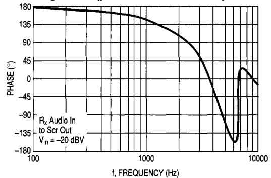
Figure 74. R x Audio Inband Phase Response
