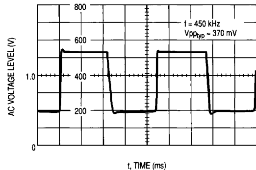
Figure 55. Typical Limiter Output Waveform with Ceramic Resonator
