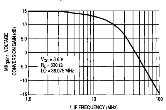
Figure 22. First IF Bandwidth
