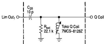
Figure 50. Quadrature Detector Demodulator Schematic
