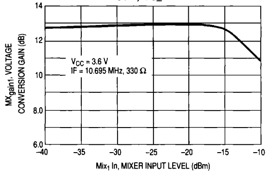
Figure 18. First Mixer Voltage Conversion Gain, IP3_bit = 1
