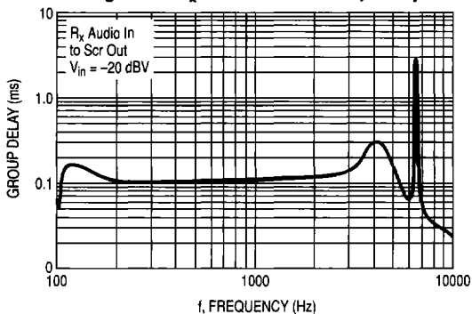
Figure 75. R x Audio Inband Group Delay
