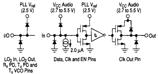
Figure 94. PLL I/O Pin Simplified Schematics
