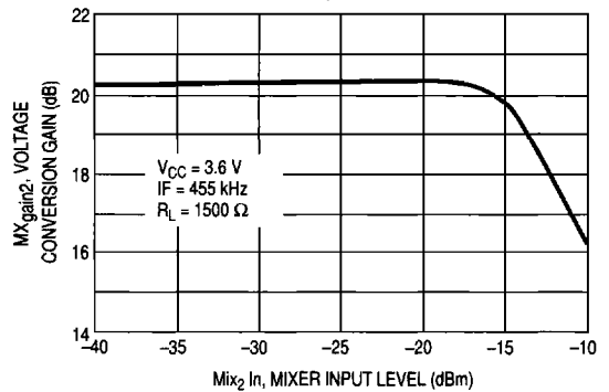
Figure 27. Second Mixer Conversion Gain, IP3_bit = 1
