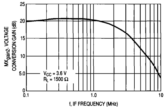
Figure 31. Second IF Bandwidth
