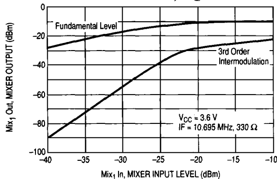
Figure 19. First Mixer Output Level and Intermodulation, IP3_bit = 0
