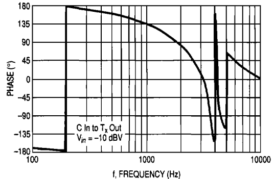
Figure 85. T x Audio Inband Phase Response
