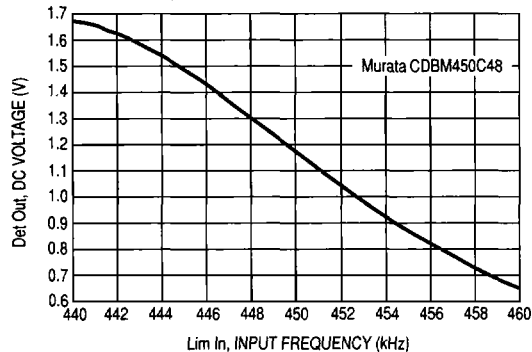
Figure 54. S-Curve of Limiter Discriminator with Ceramic Resonator
