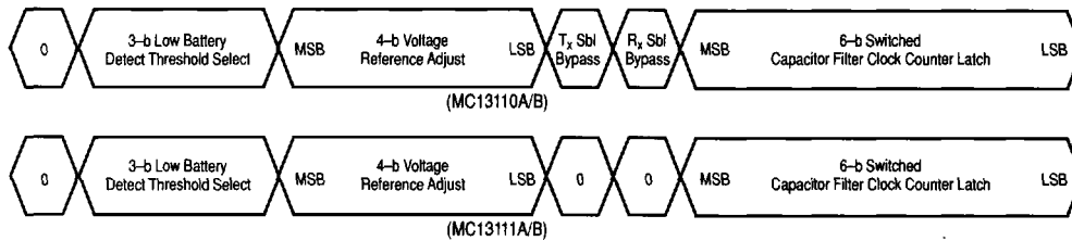
Figure 127. Clock Divider/Voltage Adjust Latch Bits
