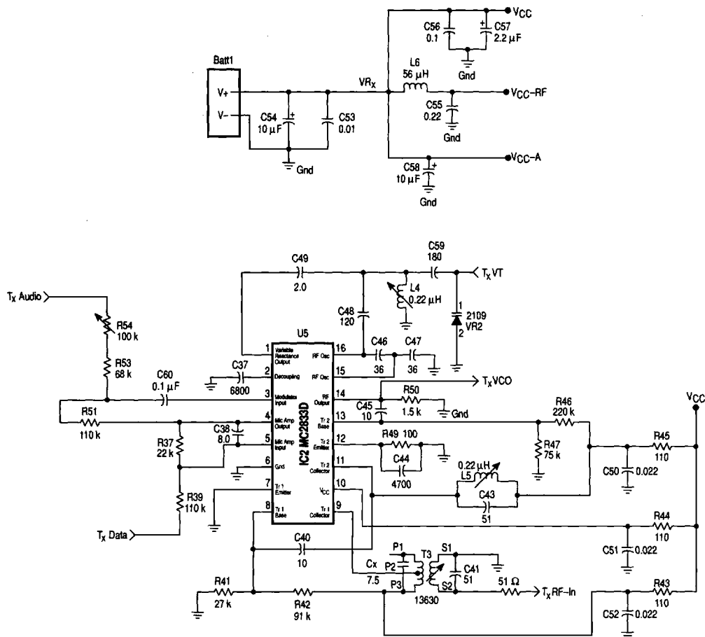
Figure 140. Basic Cordless Telephone Transceiver Application Circuit (continued)
