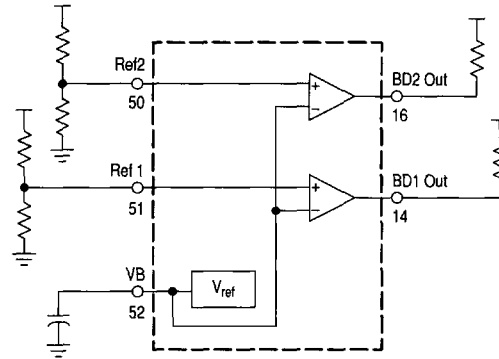
Non-Programmable Threshold Mode: 52-QFP Package
