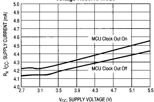
Figure 5. Current versus Supply Voltage Receive Mode
