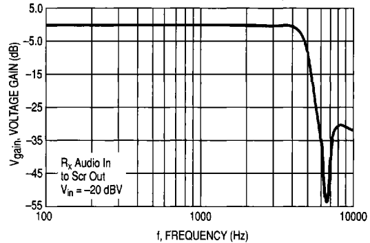
Figure 72. R x Audio Inband Frequency Response
