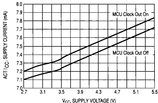
Figure 6. Current versus Supply Voltage Active Mode
