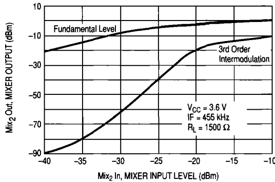
Figure 28. Second Mixer Output Level and Intermodulation, IP3_bit = 0
