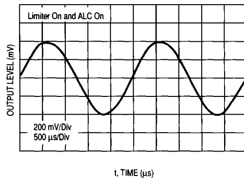
Figure 93. T x Audio Output Response
