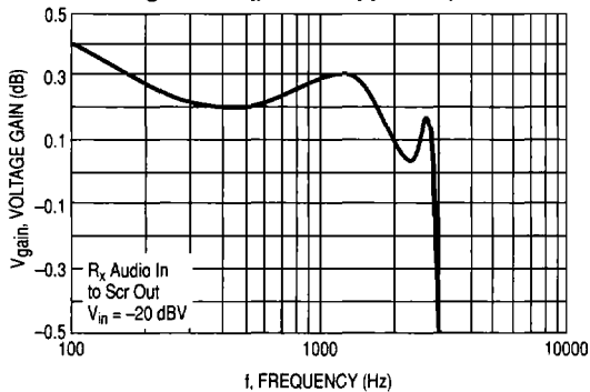
Figure 73. R x Audio Ripple Response
