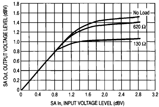
Figure 79. R x Audio Speaker Amplifier Drive
