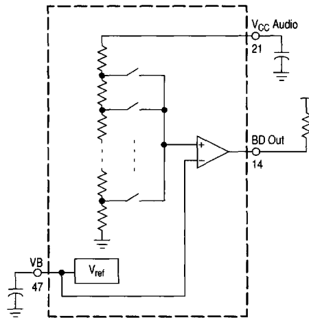
Programmable Threshold Mode: 48-LQFP Package
