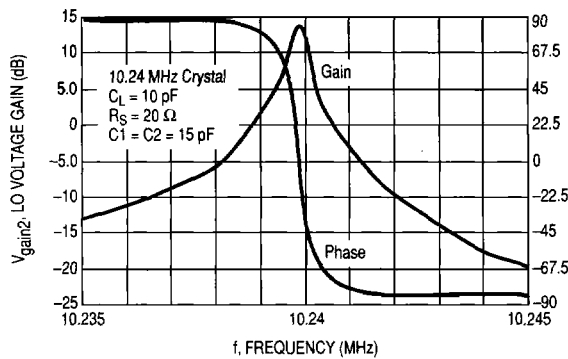
Figure 41. Second LO Gain/Phase @ -10 dBm
