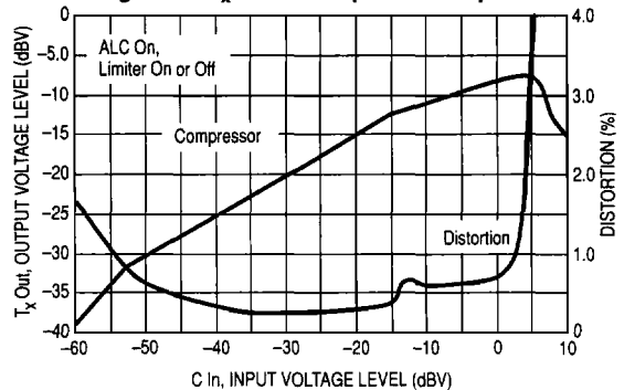
Figure 87. T x Audio Compressor Response
