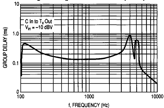
Figure 86. T x Audio Inband Group Delay
