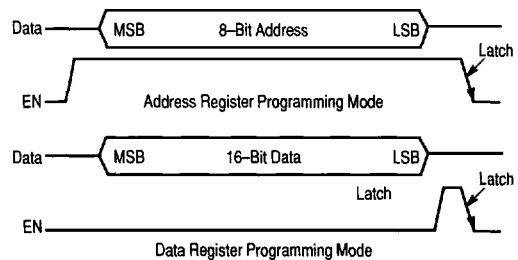
Figure 107. Microprocessor Interface Programming Mode Diagrams
