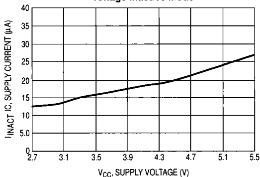
Figure 3. Current versus Supply Voltage Inactive Mode
