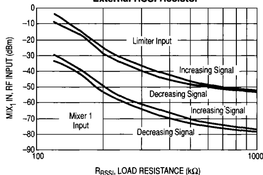
Figure 57. Carrier Detect Threshold versus External RSSI Resistor
