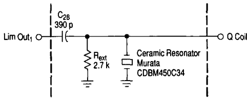
Figure 51. Ceramic Resonator Demodulator Schematic with Murata CDBM450C48
