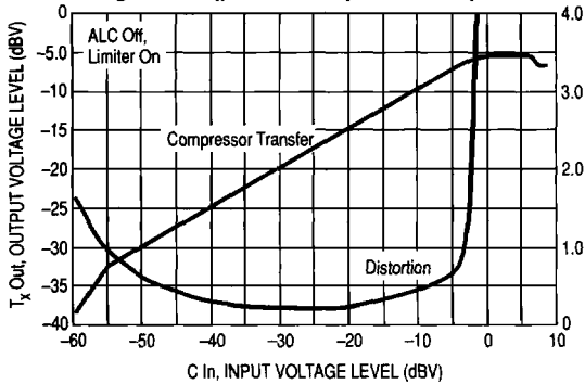
Figure 88. T x Audio Compressor Response
