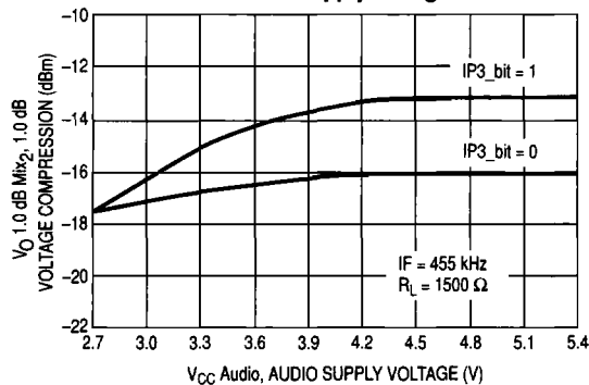
Figure 30. Second Mixer Compression versus Supply Voltage
