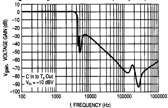
Figure 82. T x Audio Wideband Frequency Response
