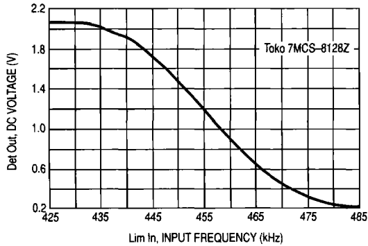
Figure 52. S-Curve of Limiter Discriminator with Quadrature Coil
