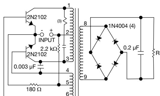
TEST CIRCUIT NUMBER 6
