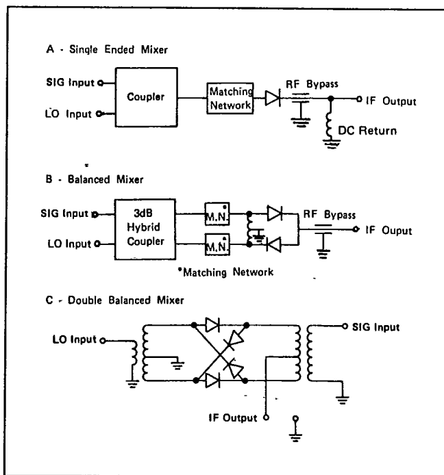
Figure 3. Typical Mixer Circuits
