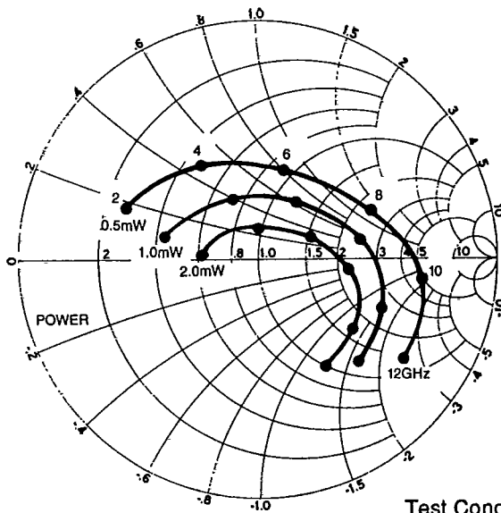
Typical DMB5827 Low Drive X-Band Mixer Diode Admittance Characteristics
