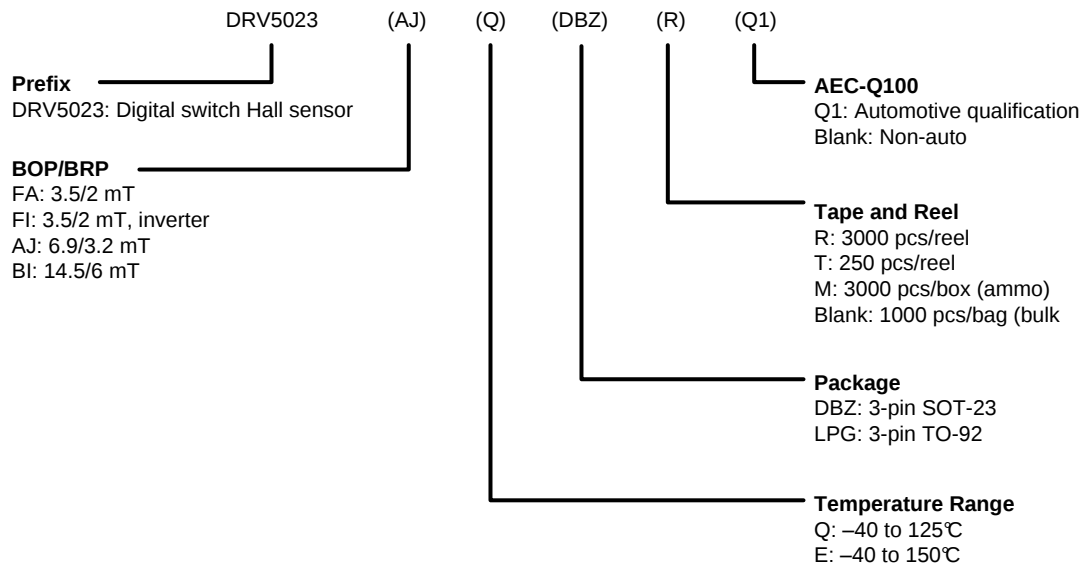
Figure 26. Device Nomenclature
