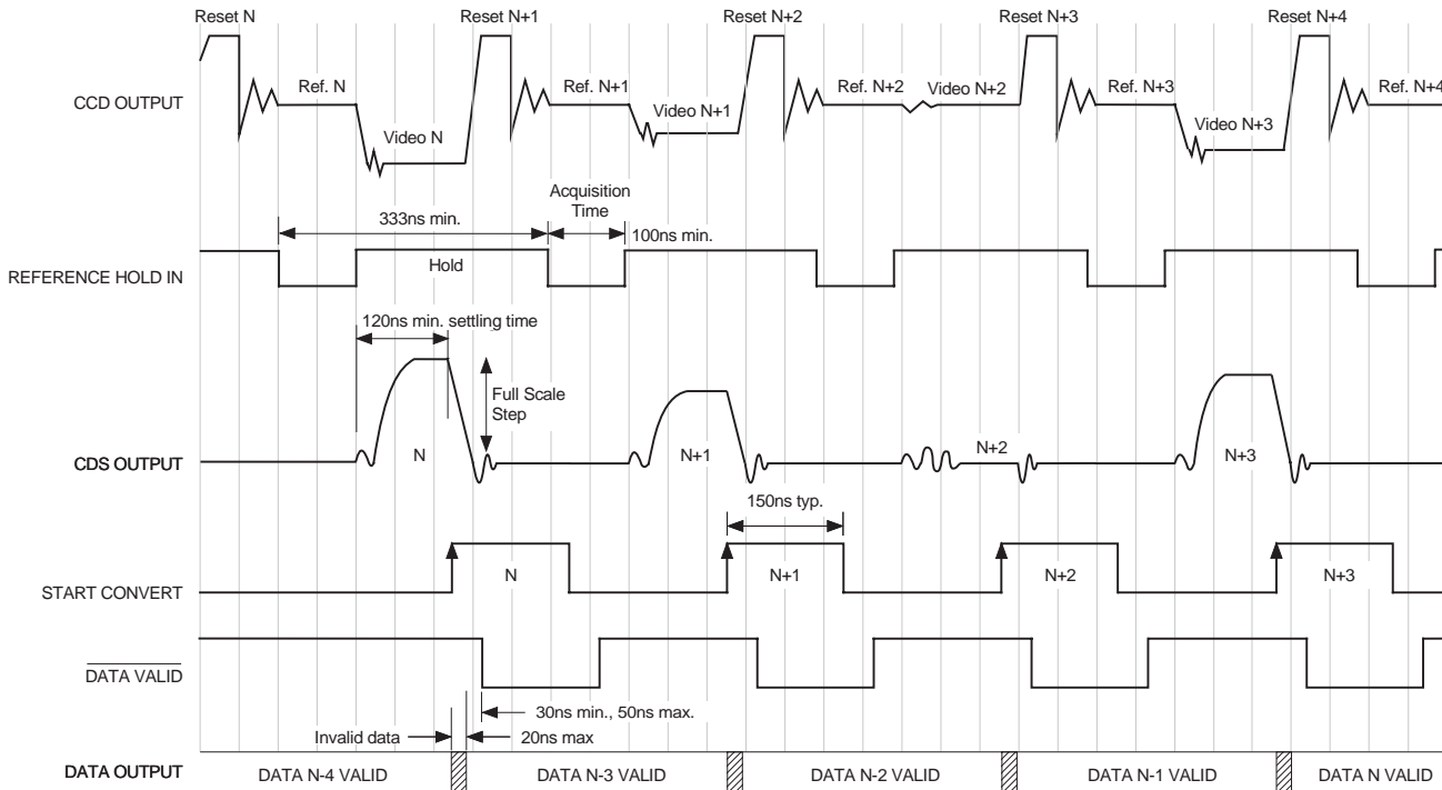
Figure 11. ADCDS-1403 Timing Diagram
