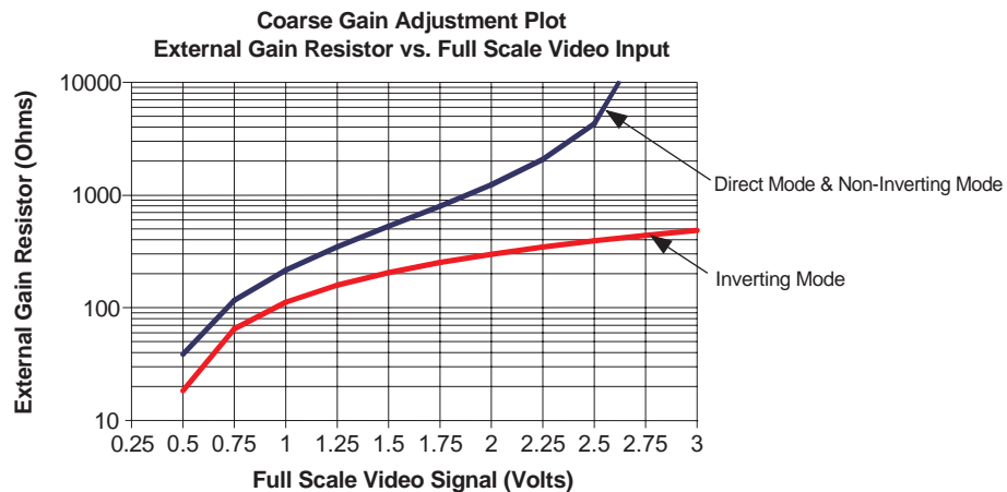
Figure 4. Coarse Gain Adjustment Plot
