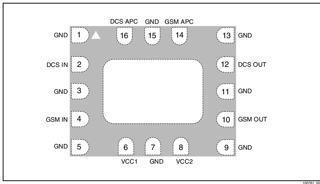
Figure 3. RM008 Pin Configuration–16-Pin Leadless PAM (Top View)
