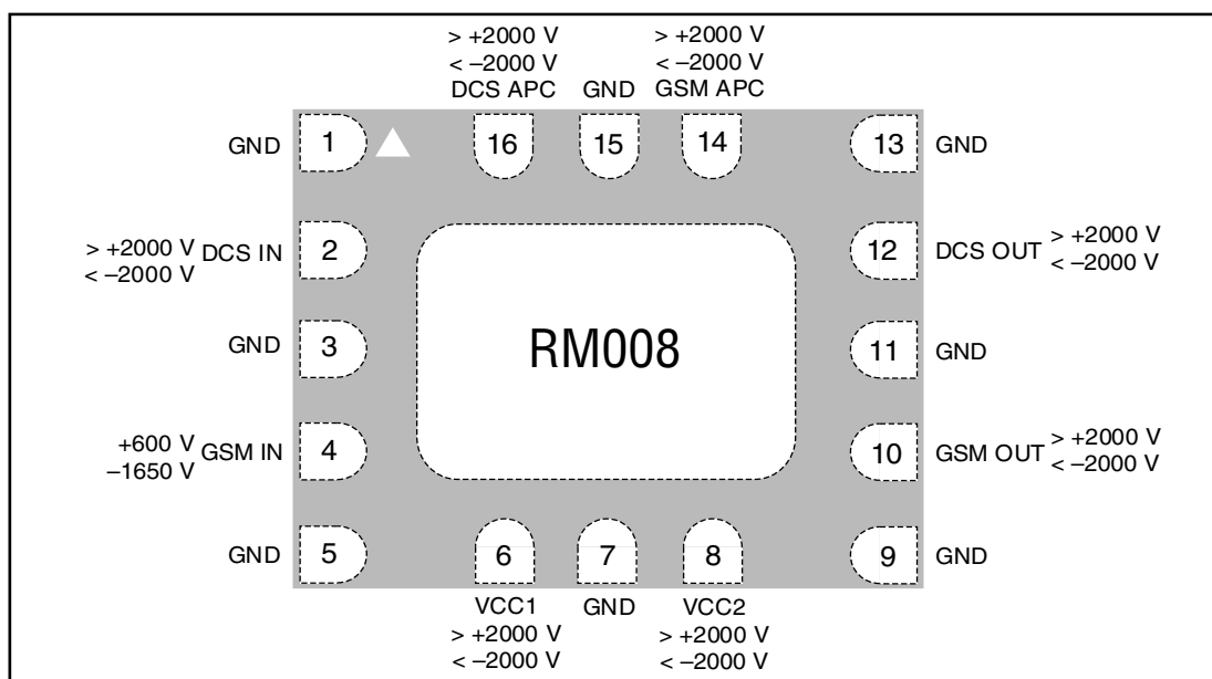
Figure 6. ESD Sensitivity Ares (Top View)
